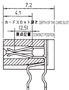
奇数ピン位置 POSITION OF ODD-NUMBERED PINS
