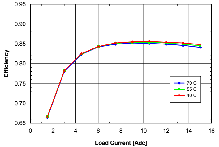
Fig. 1.8V.6: Efficiency vs. load current and ambient temperature for ASQ24T/S15018 converter mounted vertically with V_{in} = 24\text{V} and air flowing from pin 3 to pin 1 at a rate of 200 LFM (1.0 m/s).
