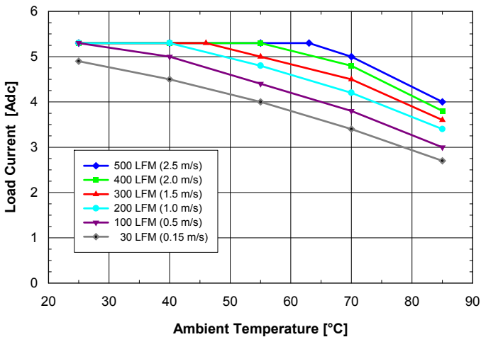
Fig. 8.0V.1: Available load current vs. ambient air temperature and airflow rates for ASQ24T05080 converter with D height pins mounted vertically with V_{in} = 24\text{ V} , air flowing from pin 3 to pin 1 and maximum FET temperature \leq 120^\circ\text{C} .
