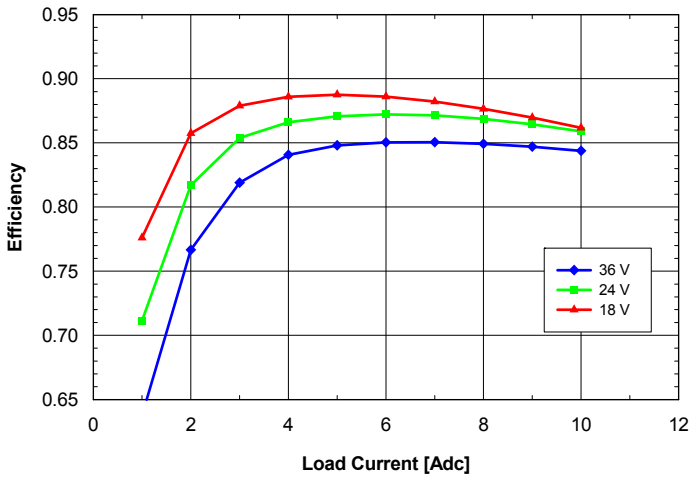
Fig. 5.0V.5: Efficiency vs. load current and input voltage for ASQ24T/S10050 converter mounted vertically with air flowing from pin 3 to pin 1 at a rate of 300 LFM (1.5 m/s) and T_a = 25^\circ\text{C} .
