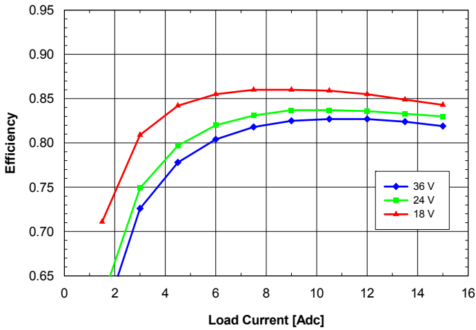
Fig. 1.5V.5: Efficiency vs. load current and input voltage for ASQ24T/S15015 converter mounted vertically with air flowing from pin 3 to pin 1 at a rate of 300 LFM (1.5 m/s) and T_a = 25^\circ\text{C} .
