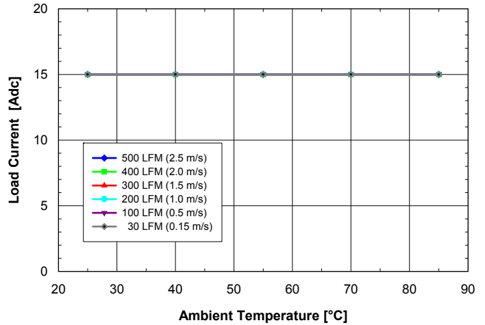
Fig. 1.2V.4: Available load current vs. ambient temperature and airflow rates for ASQ24S15012 converter mounted horizontally with V_{in} = 24V , air flowing from pin 3 to pin 1 and maximum FET temperature \leq 120^{\circ}C .
