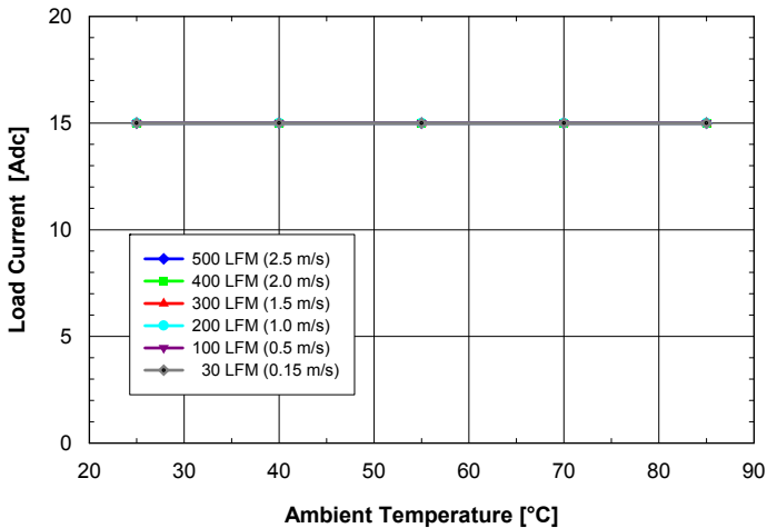
Fig. 1.2V.3: Available load current vs. ambient temperature and airflow rates for ASQ24S15012 converter mounted vertically with V_{in} = 24V , air flowing from pin 3 to pin 1 and maximum FET temperature \leq 120^{\circ}C .
