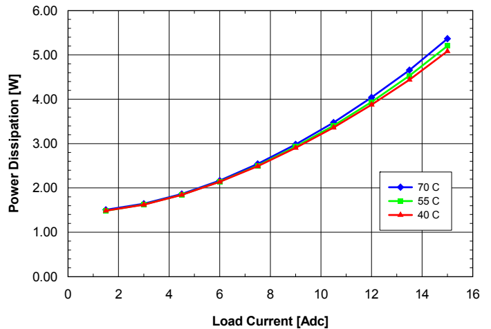
Fig. 2.0V.8: Power dissipation vs. load current and ambient temperature for ASQ24T/S15020 converter mounted vertically with V_{in} = 24\text{V} and air flowing from pin 3 to pin 1 at a rate of 200 LFM (1.0 m/s).
