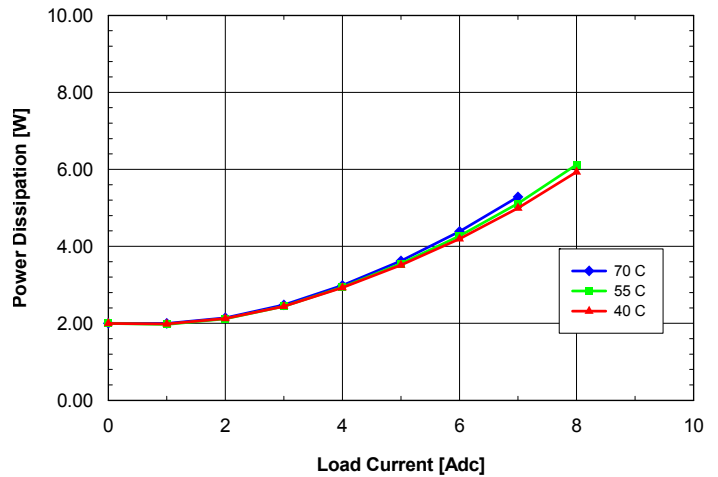
Fig. 6.0V.8: Power dissipation vs. load current and ambient temperature for ASQ24T/S08060 converter mounted vertically with V_{in} = 24\text{V} and air flowing from pin 3 to pin 1 at a rate of 200 LFM (1.0 m/s).
