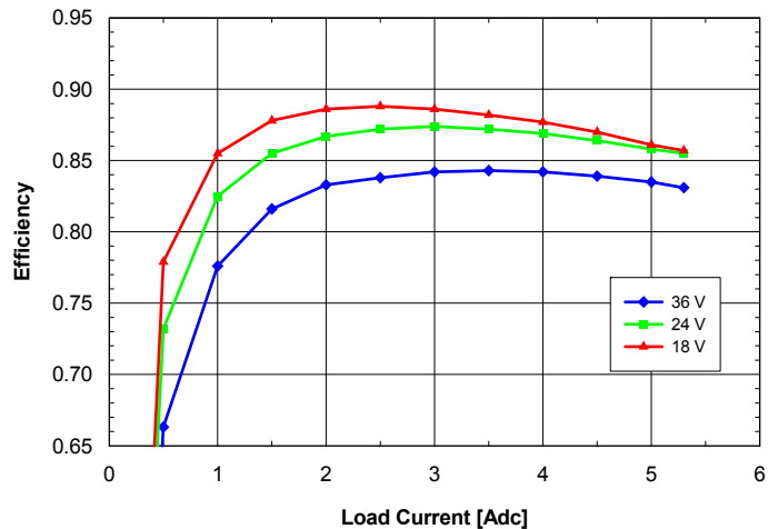
Fig. 8.0V.2: Efficiency vs. load current and input voltage for ASQ24T/S05080 converter mounted vertically with air flowing from pin 3 to pin 1 at a rate of 300 LFM (1.5 m/s) and T_a = 25^\circ\text{C} .
