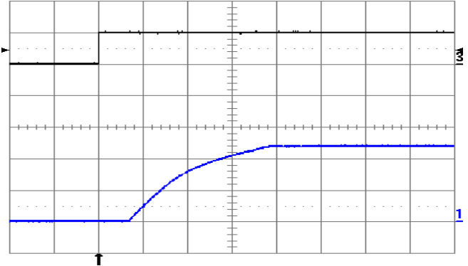
Fig. 12V.10: Turn-on transient at full rated load current (resistive) plus 1,000 \mu F at V_{in} = 24V , triggered via ON/OFF pin. Top trace: ON/OFF signal (5 V/div.). Bottom trace: output voltage (5 V/div.). Time scale: 2 ms/div.
