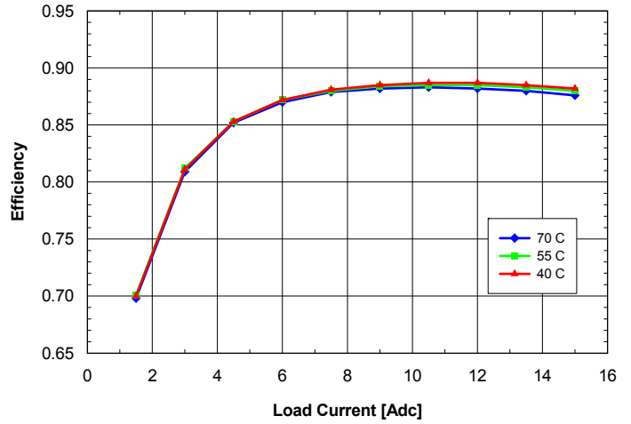
Fig. 3.3V.6: Efficiency vs. load current and ambient temperature for ASQ24T/S15033 converter mounted vertically with V_{in} = 24\text{V} and air flowing from pin 3 to pin 1 at a rate of 200 LFM (1.0 m/s).
