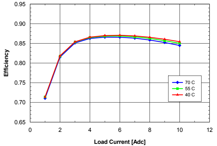
Fig. 5.0V.6: Efficiency vs. load current and ambient temperature for ASQ24T/S10050 converter mounted vertically with V_{in} = 24\text{V} and air flowing from pin 3 to pin 1 at a rate of 200 LFM (1.0 m/s).
