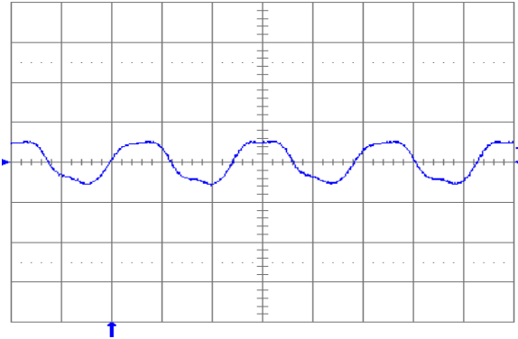
Fig. 6.0V.13: Output voltage ripple (50 mV/div.) at full rated load current into a resistive load with C_o = 10 \mu\text{F} tantalum + 1\mu\text{F} ceramic and V_{in} = 24\text{V} . Time scale: 1 \mu\text{s}/\text{div} .
