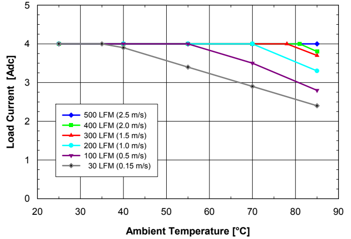
Fig. 12V.2: Available load current vs. ambient air temperature and airflow rates for ASQ24T04120 converter with B height pins mounted horizontally with V_{in} = 24V , air flowing from pin 3 to pin 1 and maximum FET temperature \leq 120^{\circ}C .
