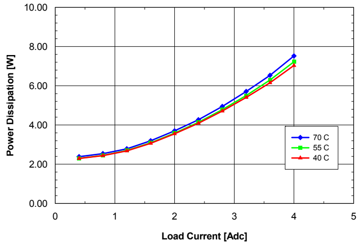
Fig. 12V.8: Power dissipation vs. load current and ambient temperature for ASQ24T/S04120 converter mounted vertically with V_{in} = 24\text{V} and air flowing from pin 3 to pin 1 at a rate of 200 LFM (1.0 m/s).
