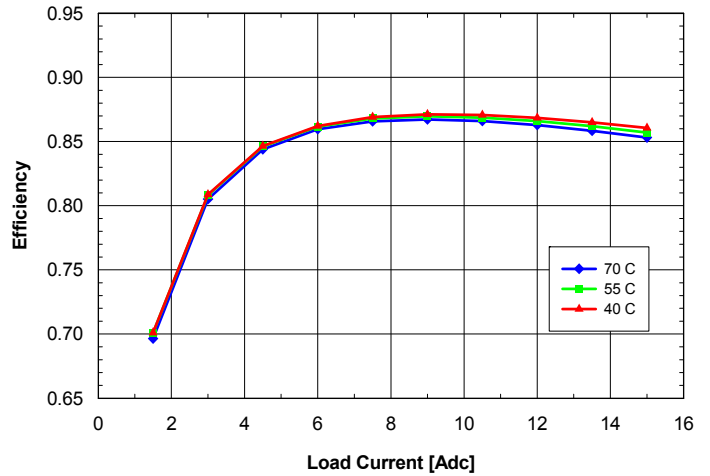
Fig. 2.5V.6: Efficiency vs. load current and ambient temperature for ASQ24T/S15025 converter mounted vertically with V_{in} = 24\text{V} and air flowing from pin 3 to pin 1 at a rate of 200 LFM (1.0 m/s).
