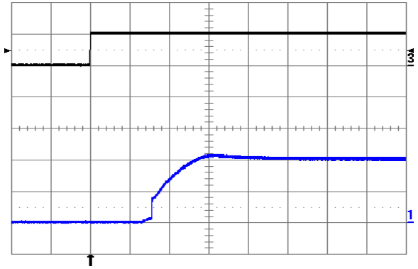
Fig. 1.0V.10: Turn-on transient at full rated load current (resistive) plus 10,000\mu F at V_{in} = 24V , triggered via ON/OFF pin. Top trace: ON/OFF signal (5 V/div.). Bottom trace: output voltage (0.5 V/div.). Time scale: 1 ms/div.
