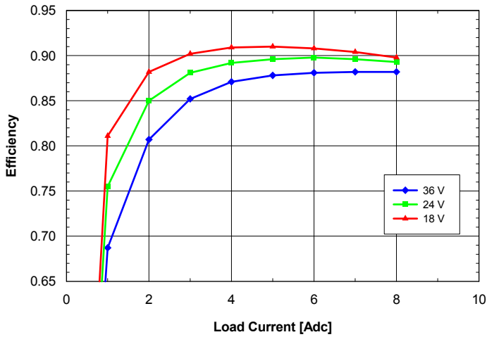
Fig. 6.0V.5: Efficiency vs. load current and input voltage for ASQ24T/S08060 converter mounted vertically with air flowing from pin 3 to pin 1 at a rate of 300 LFM (1.5 m/s) and T_a = 25^\circ\text{C} .
