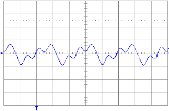
Fig. 2.0V.13: Output voltage ripple (20 mV/div.) at full rated load current into a resistive load with C_o = 10 \mu\text{F} tantalum + 1\mu\text{F} ceramic and V_{in} = 24\text{V} . Time scale: 1 \mu\text{s}/\text{div} .
