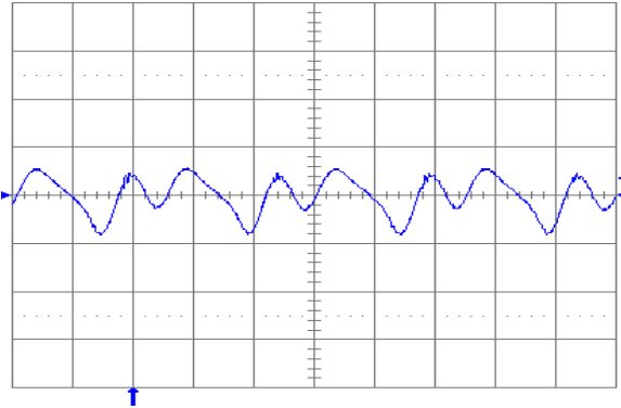
Fig. 1.0V.13: Output voltage ripple (20 mV/div.) at full rated load current into a resistive load with C_o = 10 \mu\text{F} tantalum + 1\mu\text{F} ceramic and V_{in} = 24\text{V} . Time scale: 1 \mu\text{s}/\text{div} .
