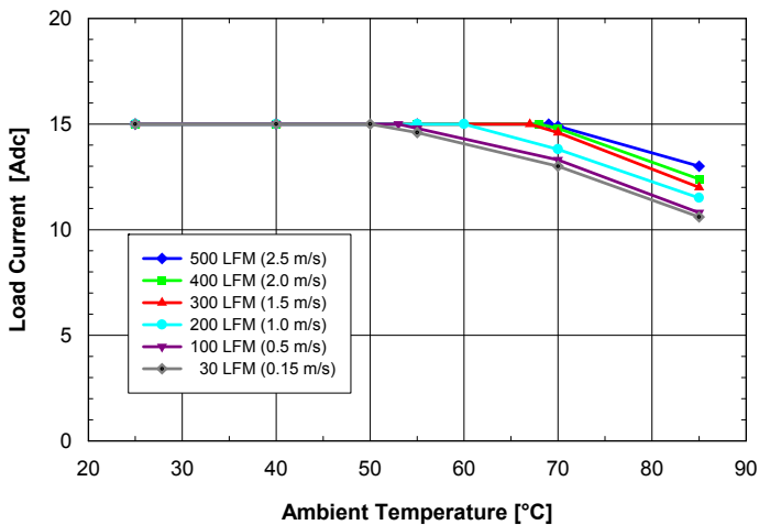
Fig. 2.5V.3: Available load current vs. ambient temperature and airflow rates for ASQ24S15025 converter mounted vertically with V_{in} = 24V , air flowing from pin 3 to pin 1 and maximum FET temperature \leq 120^{\circ}C .
