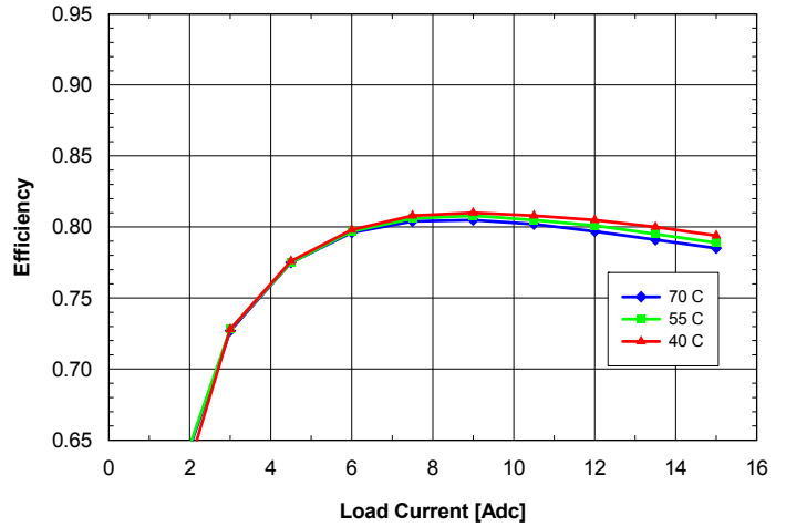
Fig. 1.0V.6: Efficiency vs. load current and ambient temperature for ASQ24T/S15010 converter mounted vertically with V_{in} = 24\text{V} and air flowing from pin 3 to pin 1 at a rate of 200 LFM (1.0 m/s).
