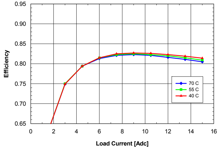
Fig. 1.2V.6: Efficiency vs. load current and ambient temperature for ASQ24T/S15012 converter mounted vertically with V_{in} = 24\text{V} and air flowing from pin 3 to pin 1 at a rate of 200 LFM (1.0 m/s).
