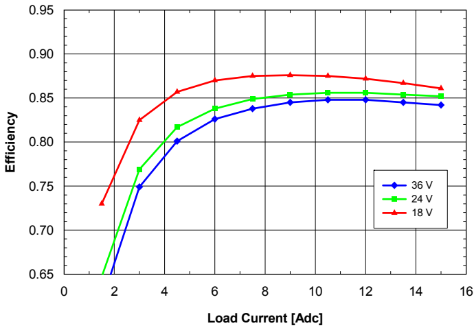
Fig. 2.0V.5: Efficiency vs. load current and input voltage for ASQ24T/S15020 converter mounted vertically with air flowing from pin 3 to pin 1 at a rate of 300 LFM (1.5 m/s) and T_a = 25^\circ\text{C} .
