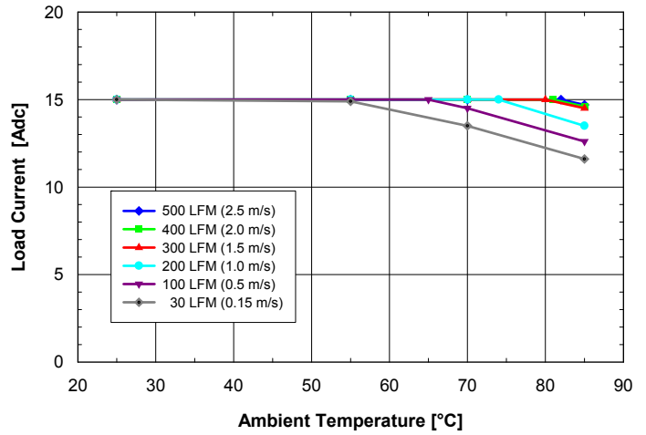
Fig. 2.5V.2: Available load current vs. ambient air temperature and airflow rates for ASQ24T15025 converter with B height pins mounted horizontally with V_{in} = 24V , air flowing from pin 3 to pin 1 and maximum FET temperature \leq 120^{\circ}C .
