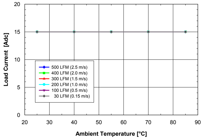
Fig. 1.0V.2: Available load current vs. ambient air temperature and airflow rates for ASQ24T15010 converter with B height pins mounted horizontally with V_{in} = 24V , air flowing from pin 3 to pin 1 and maximum FET temperature \leq 120^{\circ}C .
