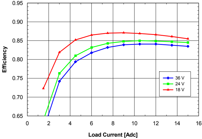
Fig. 1.8V.5: Efficiency vs. load current and input voltage for ASQ24T/S15018 converter mounted vertically with air flowing from pin 3 to pin 1 at a rate of 300 LFM (1.5 m/s) and T_a = 25^\circ\text{C} .
