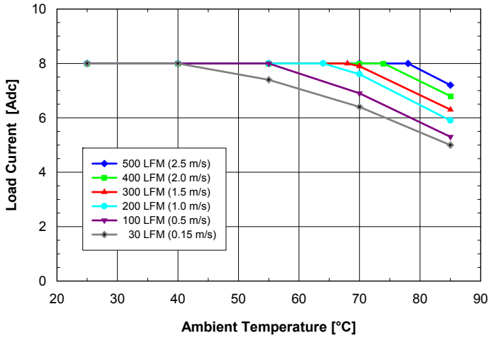
Fig. 6.0V.1: Available load current vs. ambient air temperature and airflow rates for ASQ24T08060 converter with B height pins mounted vertically with V_{in} = 24V , air flowing from pin 3 to pin 1 and maximum FET temperature \leq 120^{\circ}C .
