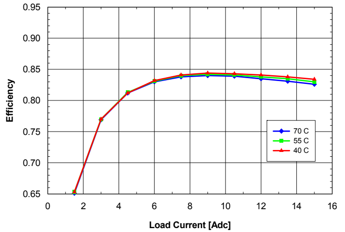
Fig. 1.5V.6: Efficiency vs. load current and ambient temperature for ASQ24T/S15015 converter mounted vertically with V_{in} = 24\text{V} and air flowing from pin 3 to pin 1 at a rate of 200 LFM (1.0 m/s).
