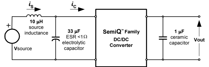
Fig. 1.2V.14: Test setup for measuring input reflected ripple currents, i_c and i_s .
