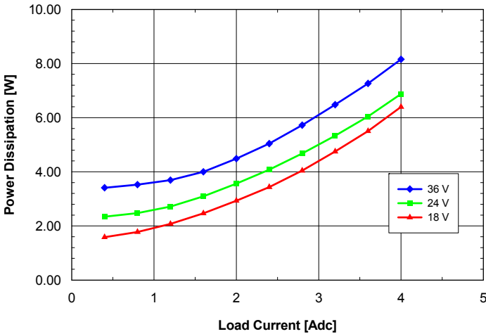
Fig. 12V.7: Power dissipation vs. load current and input voltage for ASQ24T/S04120 converter mounted vertically with air flowing from pin 3 to pin 1 at a rate of 300 LFM (1.5 m/s) and T_a = 25^\circ\text{C} .
