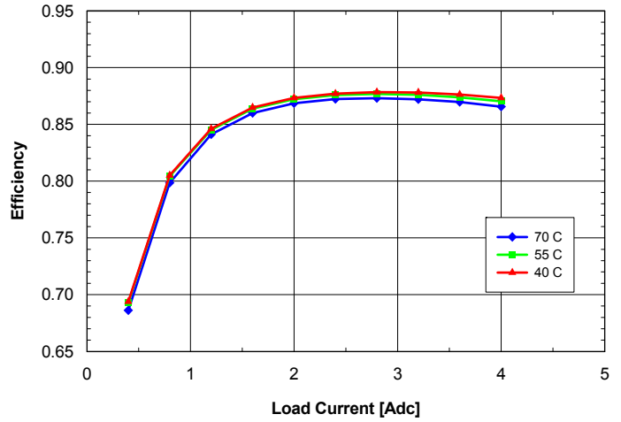
Fig. 12V.6: Efficiency vs. load current and ambient temperature for ASQ24T/S04120 converter mounted vertically with V_{in} = 24\text{V} and air flowing from pin 3 to pin 1 at a rate of 200 LFM (1.0 m/s).
