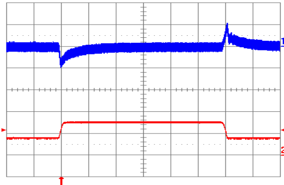
Fig. 2.5V.11: Output voltage response to load current step-change (3.75 A – 7.5 A – 3.75 A) at V_{in} = 24V . Top trace: output voltage (100 mV/div.). Bottom trace: load current (5 A/div.). Current slew rate: 0.1 A/ \mu s . C_o = 1 \mu F ceramic. Time scale: 0.2 ms/div.
