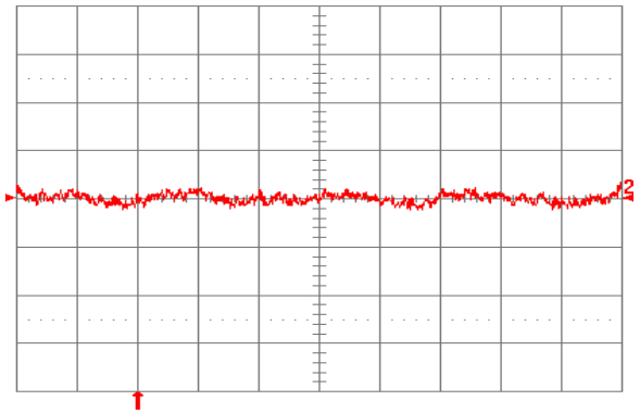
Fig. 6.0V.16: Input reflected ripple current, i_s (10 mA/div.), measured through 10 \mu\text{H} at the source at full rated load current and V_{in} = 24\text{V} . Refer to Fig. 6.0V.14 for test setup. Time scale: 1 \mu\text{s}/\text{div} .
