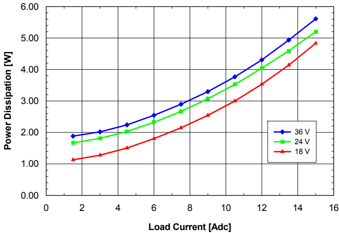
Fig. 2.0V.7: Power dissipation vs. load current and input voltage for ASQ24T/S15020 converter mounted vertically with air flowing from pin 3 to pin 1 at a rate of 300 LFM (1.5 m/s) and T_a = 25^\circ\text{C} .
