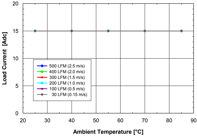
Fig. 1.5V.1: Available load current vs. ambient air temperature and airflow rates for ASQ24T15015 converter with B height pins mounted vertically with V_{in} = 24V , air flowing from pin 3 to pin 1 and maximum FET temperature \leq 120^{\circ}C .
