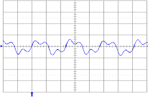
Fig. 2.5V.13: Output voltage ripple (20 mV/div.) at full rated load current into a resistive load with C_o = 10 \mu\text{F} tantalum + 1\mu\text{F} ceramic and V_{in} = 24\text{V} . Time scale: 1 \mu\text{s}/\text{div} .
