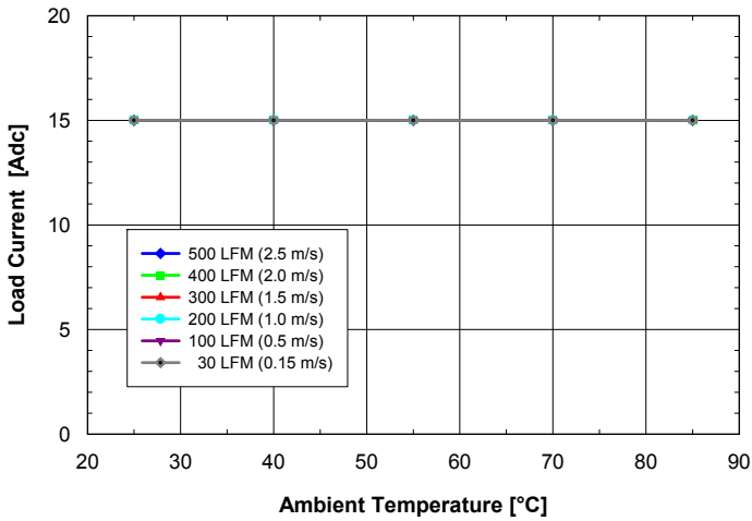
Fig. 1.0V.1: Available load current vs. ambient air temperature and airflow rates for ASQ24T15010 converter with B height pins mounted vertically with V_{in} = 24V , air flowing from pin 3 to pin 1 and maximum FET temperature \leq 120^{\circ}C .
