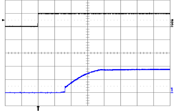
Fig. 1.8V.10: Turn-on transient at full rated load current (resistive) plus 10,000 \mu F at V_{in} = 24V , triggered via ON/OFF pin. Top trace: ON/OFF signal (5 V/div.). Bottom trace: output voltage (1 V/div.). Time scale: 1 ms/div.
