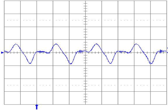
Fig. 1.5V.13: Output voltage ripple (20 mV/div.) at full rated load current into a resistive load with C_o = 10 \mu\text{F} tantalum + 1\mu\text{F} ceramic and V_{in} = 24\text{V} . Time scale: 1 \mu\text{s}/\text{div} .
