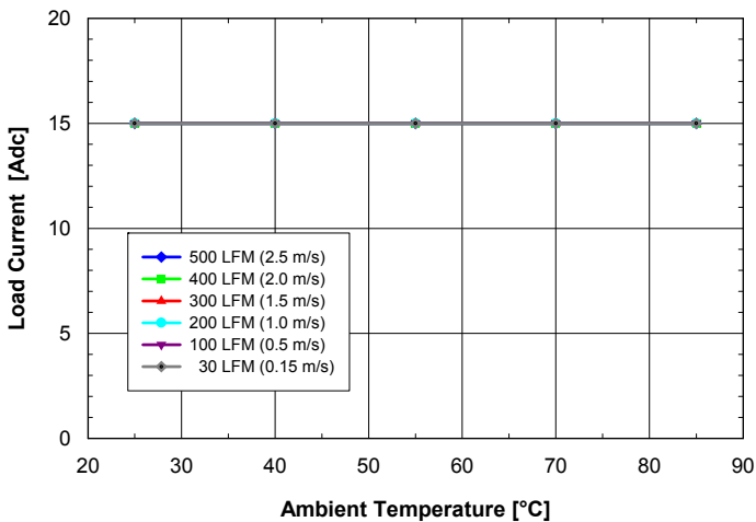
Fig. 1.0V.3: Available load current vs. ambient temperature and airflow rates for ASQ24S15010 converter mounted vertically with V_{in} = 24V , air flowing from pin 3 to pin 1 and maximum FET temperature \leq 120^{\circ}C .
