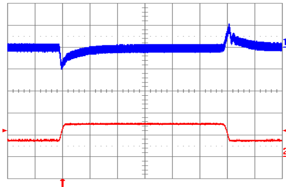
Fig. 2.0V.11: Output voltage response to load current step-change (3.75A – 7.5A – 3.75A) at V_{in} = 24V . Top trace: output voltage (100 mV/div.). Bottom trace: load current (5 A/div.). Current slew rate: 0.1 A/ \mu s . C_o = 1 \mu F ceramic. Time scale: 0.2 ms/div.
