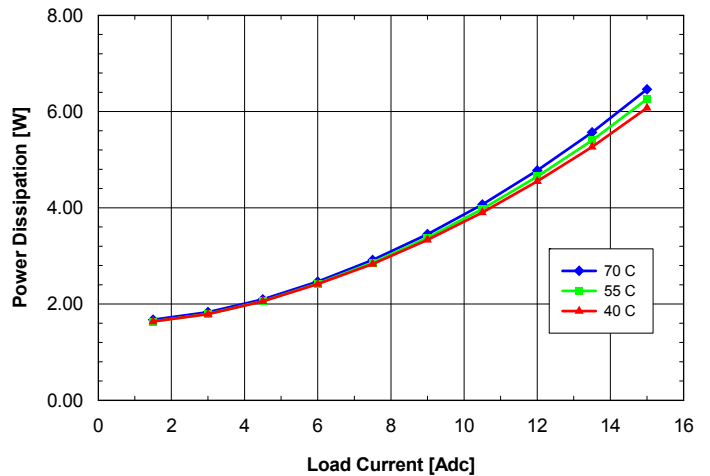
Fig. 2.5V.8: Power dissipation vs. load current and ambient temperature for ASQ24T/S15025 converter mounted vertically with V_{in} = 24\text{V} and air flowing from pin 3 to pin 1 at a rate of 200 LFM (1.0 m/s).
