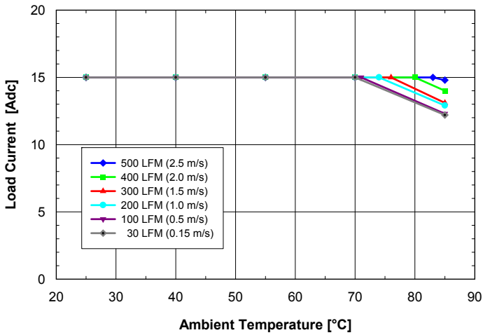
Fig. 2.5V.1: Available load current vs. ambient air temperature and airflow rates for ASQ24T15025 converter with B height pins mounted vertically with V_{in} = 24V , air flowing from pin 3 to pin 1 and maximum FET temperature \leq 120^{\circ}C .
