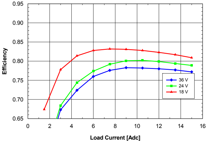
Fig. 1.0V.5: Efficiency vs. load current and input voltage for ASQ24T/S15010 converter mounted vertically with air flowing from pin 3 to pin 1 at a rate of 300 LFM (1.5 m/s) and T_a = 25^\circ\text{C} .
