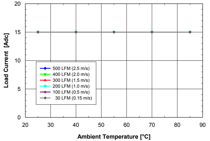
Fig. 1.2V.2: Available load current vs. ambient air temperature and airflow rates for ASQ24T15012 converter with B height pins mounted horizontally with V_{in} = 24V , air flowing from pin 3 to pin 1 and maximum FET temperature \leq 120^{\circ}C .
