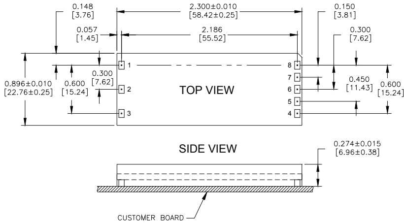
ASQ24S Pinout (Surface Mount)
