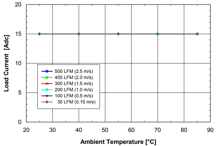
Fig. 1.0V.4: Available load current vs. ambient temperature and airflow rates for ASQ24S15010 converter mounted horizontally with V_{in} = 24V , air flowing from pin 3 to pin 1 and maximum FET temperature \leq 120^{\circ}C .
