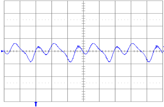
Fig. 1.2V.13: Output voltage ripple (20 mV/div.) at full rated load current into a resistive load with C_o = 10 \mu\text{F} tantalum + 1\mu\text{F} ceramic and V_{in} = 24\text{V} . Time scale: 1 \mu\text{s}/\text{div} .
