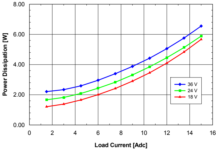
Fig. 2.5V.7: Power dissipation vs. load current and input voltage for ASQ24T/S15025 converter mounted vertically with air flowing from pin 3 to pin 1 at a rate of 300 LFM (1.5 m/s) and T_a = 25^\circ\text{C} .
