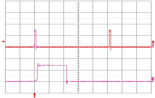
Fig. 5.0V.18: Load current (top trace, 10 A/div., 20 ms/div.) into a 10 mΩ short circuit during restart, at V in = 24V. Bottom trace (10 A/div., 1 ms/div.) is an expansion of the on-time portion of the top trace.
