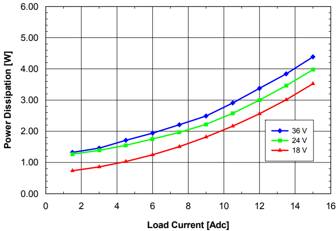
Fig. 1.0V.7: Power dissipation vs. load current and input voltage for ASQ24T/S15010 converter mounted vertically with air flowing from pin 3 to pin 1 at a rate of 300 LFM (1.5 m/s) and T_a = 25^\circ\text{C} .
