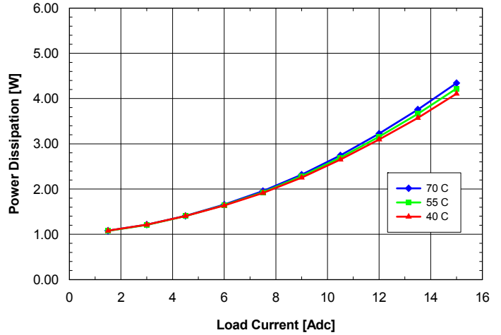
Fig. 1.2V.8: Power dissipation vs. load current and ambient temperature for ASQ24T/S15012 converter mounted vertically with V_{in} = 24\text{V} and air flowing from pin 3 to pin 1 at a rate of 200 LFM (1.0 m/s).
