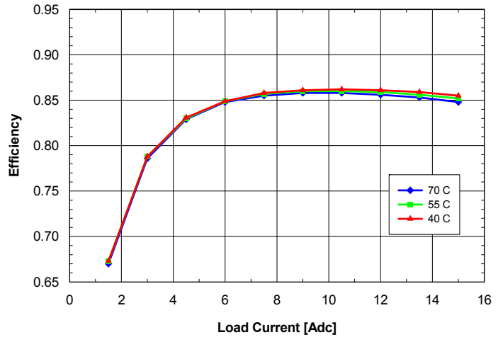
Fig. 2.0V.6: Efficiency vs. load current and ambient temperature for ASQ24T/S15020 converter mounted vertically with V_{in} = 24\text{V} and air flowing from pin 3 to pin 1 at a rate of 200 LFM (1.0 m/s).
