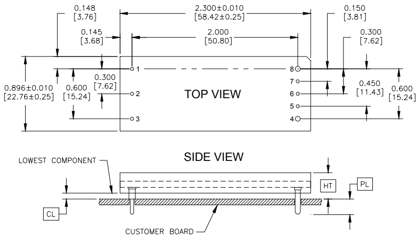
ASQ24T Pinout (Through-hole)
