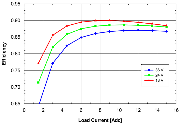
Fig. 3.3V.5: Efficiency vs. load current and input voltage for ASQ24T/S15033 converter mounted vertically with air flowing from pin 3 to pin 1 at a rate of 300 LFM (1.5 m/s) and T_a = 25^\circ\text{C} .
