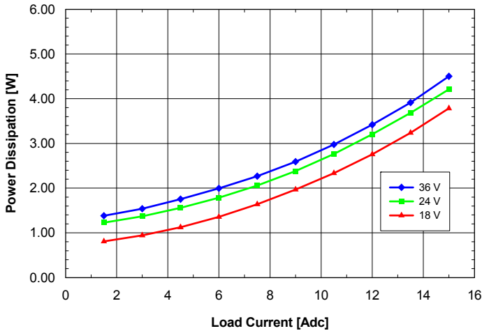
Fig. 1.2V.7: Power dissipation vs. load current and input voltage for ASQ24T/S15012 converter mounted vertically with air flowing from pin 3 to pin 1 at a rate of 300 LFM (1.5 m/s) and T_a = 25^\circ\text{C} .
