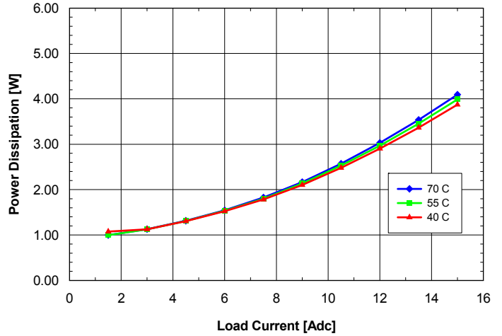
Fig. 1.0V.8: Power dissipation vs. load current and ambient temperature for ASQ24T/S15010 converter mounted vertically with V_{in} = 24\text{V} and air flowing from pin 3 to pin 1 at a rate of 200 LFM (1.0 m/s).
