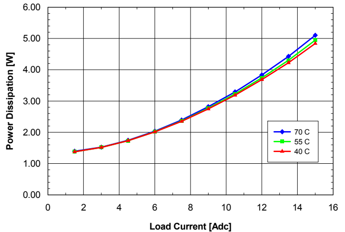
Fig. 1.8V.8: Power dissipation vs. load current and ambient temperature for ASQ24T/S15018 converter mounted vertically with V_{in} = 24\text{V} and air flowing from pin 3 to pin 1 at a rate of 200 LFM (1.0 m/s).
