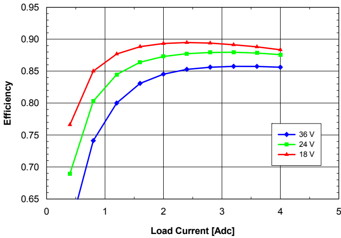
Fig. 12V.5: Efficiency vs. load current and input voltage for ASQ24T/S04120 converter mounted vertically with air flowing from pin 3 to pin 1 at a rate of 300 LFM (1.5 m/s) and T_a = 25^\circ\text{C} .
