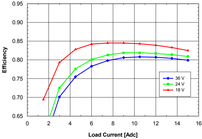
Fig. 1.2V.5: Efficiency vs. load current and input voltage for ASQ24T/S15012 converter mounted vertically with air flowing from pin 3 to pin 1 at a rate of 300 LFM (1.5 m/s) and T_a = 25^\circ\text{C} .
