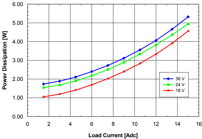
Fig. 1.8V.7: Power dissipation vs. load current and input voltage for ASQ24T/S15018 converter mounted vertically with air flowing from pin 3 to pin 1 at a rate of 300 LFM (1.5 m/s) and T_a = 25^\circ\text{C} .
