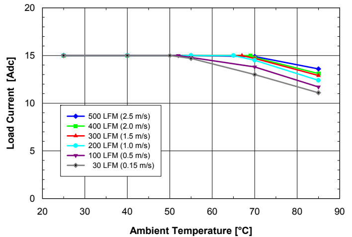
Fig. 2.5V.4: Available load current vs. ambient temperature and airflow rates for ASQ24S15025 converter mounted horizontally with V_{in} = 24V , air flowing from pin 3 to pin 1 and maximum FET temperature \leq 120^{\circ}C .
