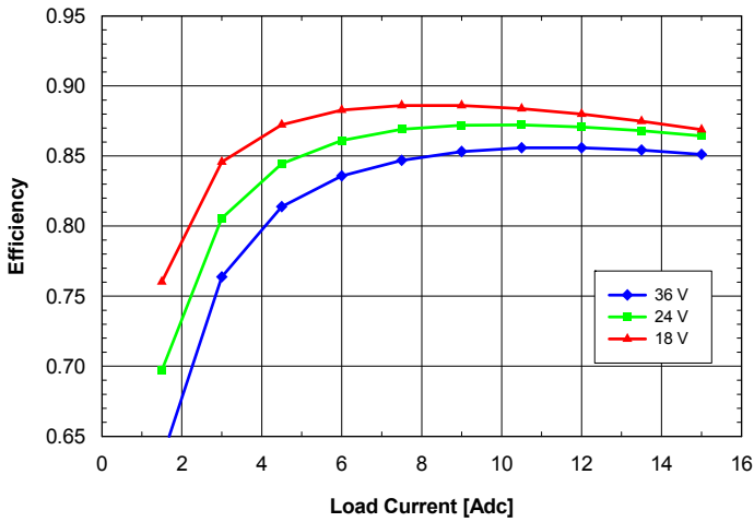
Fig. 2.5V.5: Efficiency vs. load current and input voltage for ASQ24T/S15025 converter mounted vertically with air flowing from pin 3 to pin 1 at a rate of 300 LFM (1.5 m/s) and T_a = 25^\circ\text{C} .
