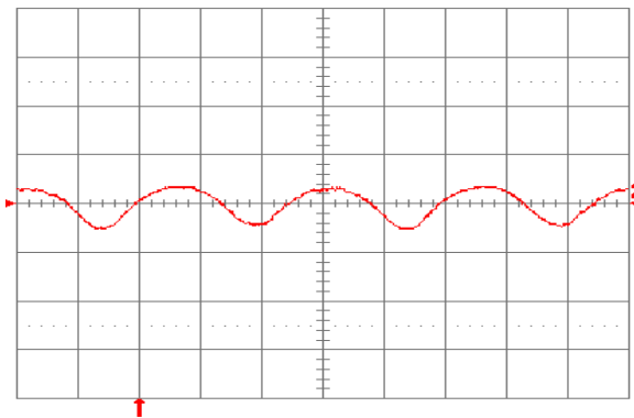
Fig. 1.2V.15: Input reflected ripple current, i_c (100 mA/div.), measured at input terminals at full rated load current and V_{in} = 24\text{V} . Refer to Fig. 1.2V.14 for test setup. Time scale: 1 \mu\text{s}/\text{div} .
