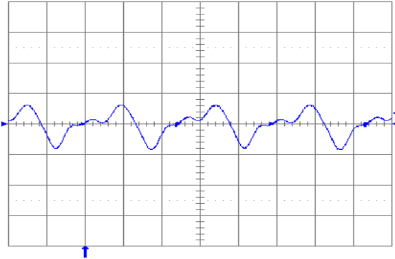
Fig. 1.8V.13: Output voltage ripple (20 mV/div.) at full rated load current into a resistive load with C_o = 10 \mu\text{F} tantalum + 1\mu\text{F} ceramic and V_{in} = 24\text{V} . Time scale: 1 \mu\text{s}/\text{div} .
