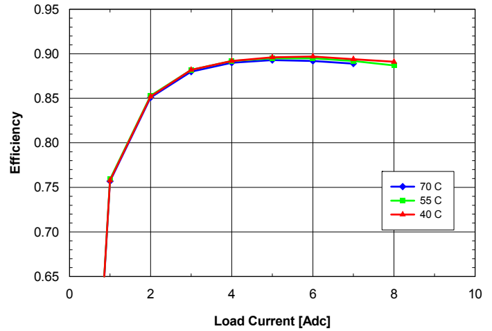
Fig. 6.0V.6: Efficiency vs. load current and ambient temperature for ASQ24T/S08060 converter mounted vertically with V_{in} = 24\text{V} and air flowing from pin 3 to pin 1 at a rate of 200 LFM (1.0 m/s).
