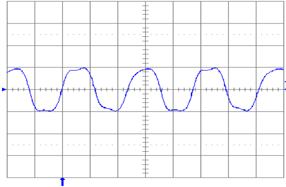
Fig. 5.0V.13: Output voltage ripple (20 mV/div.) at full rated load current into a resistive load with C_o = 10 \mu\text{F} tantalum + 1\mu\text{F} ceramic and V_{in} = 24\text{V} . Time scale: 1 \mu\text{s}/\text{div} .
