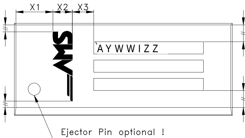
Figure 16 PB-free Marking of AS 8446
