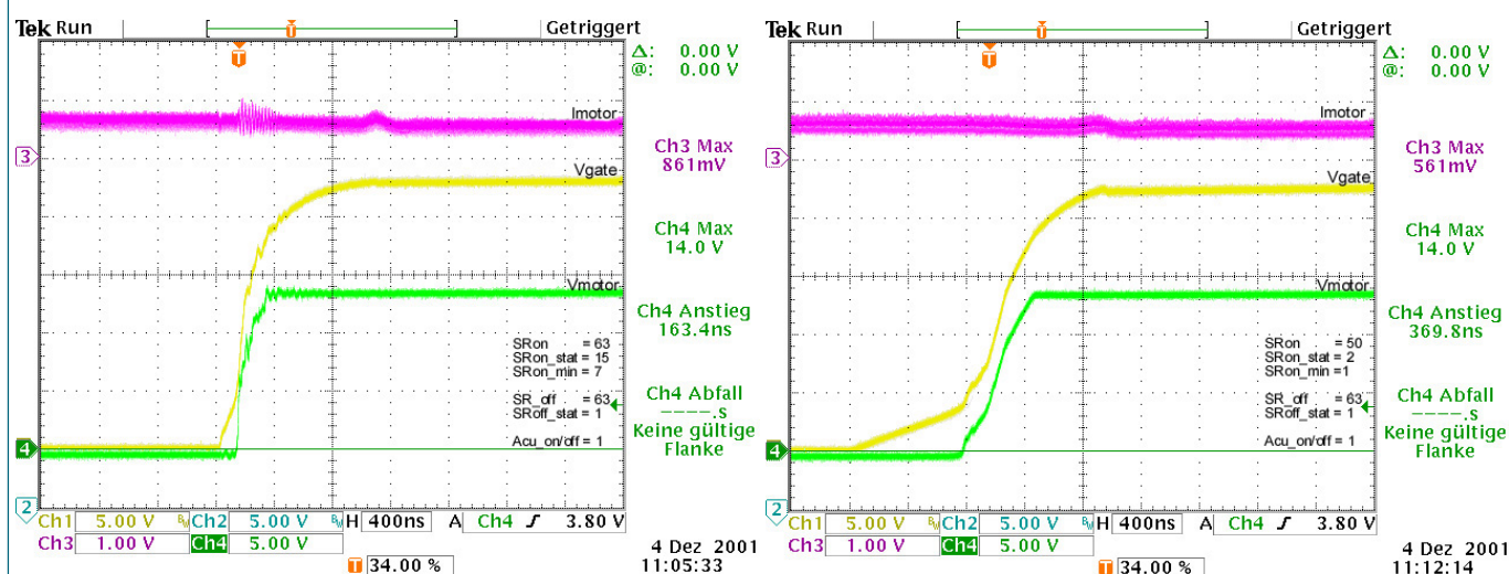
Figure 5 Rising edge of the motor voltage before and after the EMC optimization
