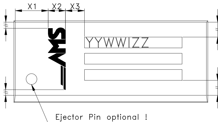
Figure 15 Marking of AS 8446
