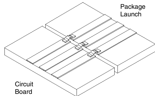
Figure 2. Microstrip Mount
