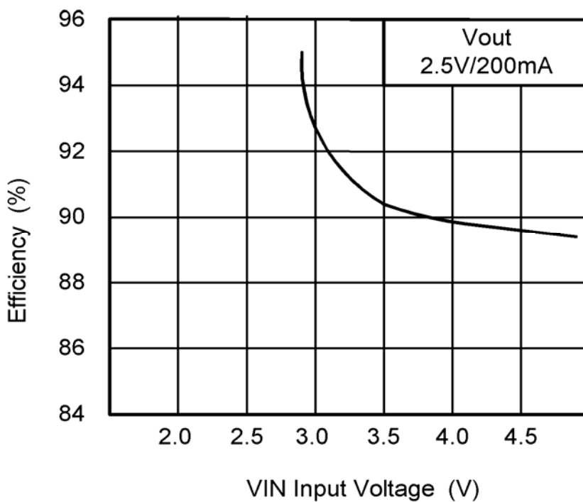
AT1391 Efficiency
