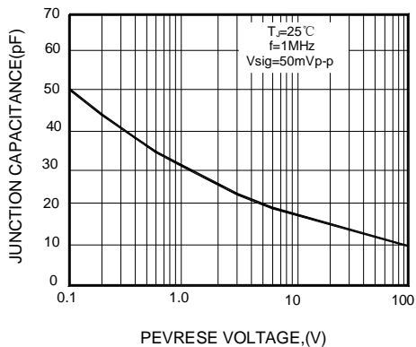
FIG.5-TYPICAL JUNCTION CAPACITANCE
