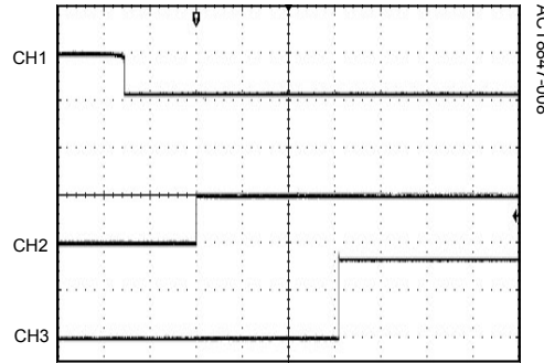
Startup of nPBIN, OUT6, nRSTO
