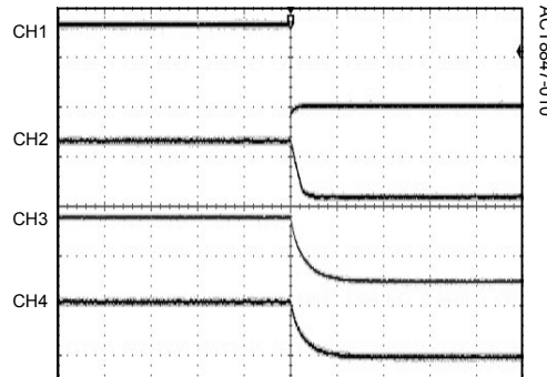
Sleep of PWREN, OUT4/2/3
