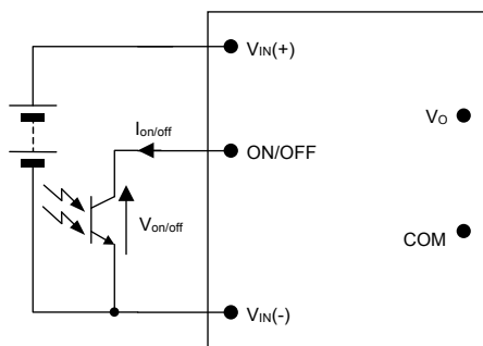
Figure 64. Remote On/Off Implementation.
