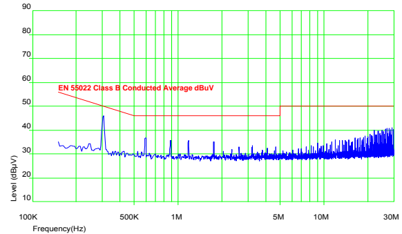
Figure 68. EMC signature using above filter, HW005A0F.
