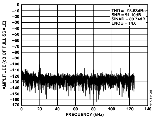
Figure 68. AD8137 Performance on Single 5 V Supply, -1.82 dBFS
