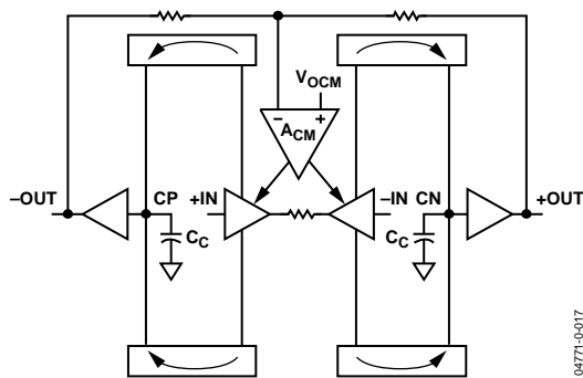
Figure 61. Block Diagram
