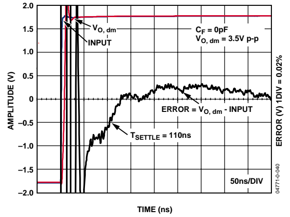
Figure 40. Settling Time (0.02%)
