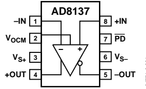
Figure 4. Pin Configuration
