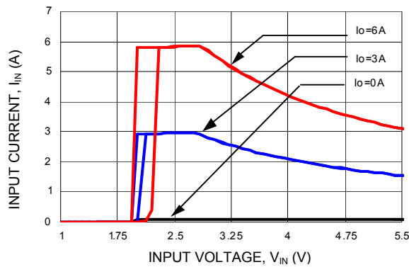
Figure 7. Input voltage vs. Input Current (Vout = 2.5Vdc).
