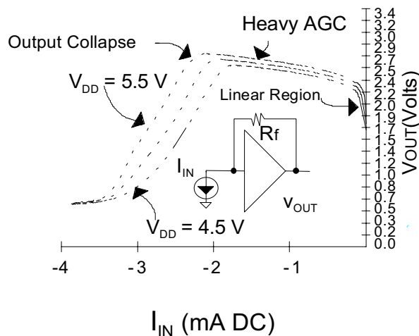
V_{OUT} vs I_{IN}
