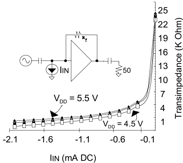
Transimpedance vs I_{IN}
