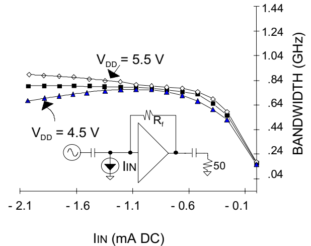
Bandwidth vs I_{IN}
