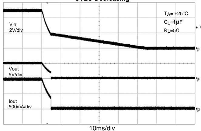
UVLO Decreasing
