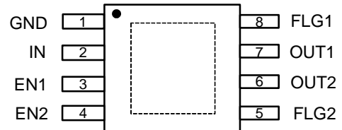
MSOP-8EP
