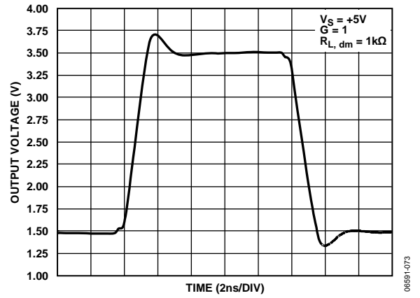
Figure 42. Large Signal V_{OCM} Pulse Response
