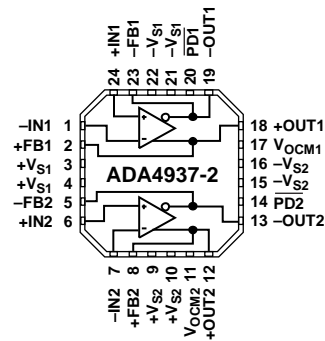
Figure 2. ADA4937-2
