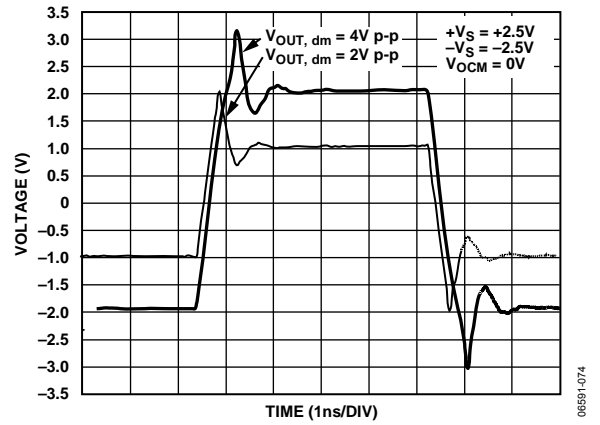
Figure 41. Large Signal Pulse Response
