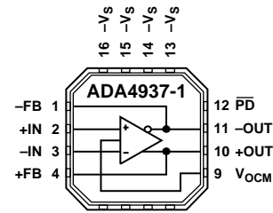
Figure 1. ADA4937-1
