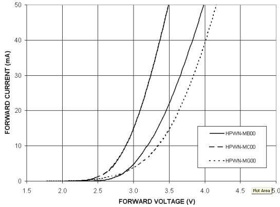
Figure 2b. Forward Current vs. Forward Voltage
