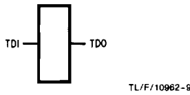
Bypass Register Scan Chain Definition
