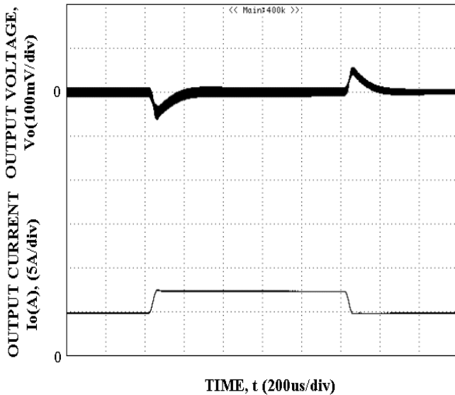
Figure 8: Output voltage response to step-change in load current (50%-75%-50% of I_{max} ; di/dt = 0.1A/\mu s ). V_{in}=48V . Load cap: 10\mu F tantalum capacitor and 1\mu F ceramic capacitor. Top trace: V_{out} (100mV/div), Bottom trace: I_{out} (5A/div). Scope measurement should be made using a BNC cable (length shorter than 20 inches). Position the load between 51 mm and 76 mm (2 inches and 3 inches) from the module.
