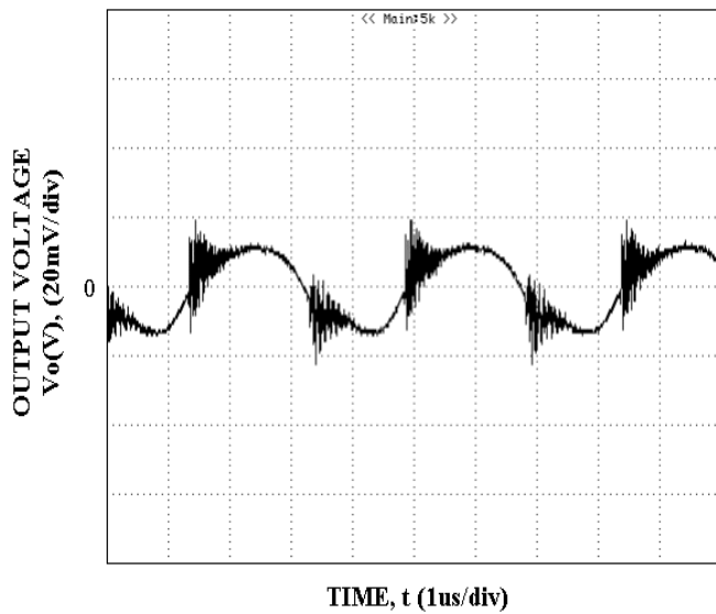
Figure 14: Output voltage ripple at nominal input Voltage ( V_{in}=48V ) and rated load current ( I_o=10A ) (20 mV/div). Load capacitance: 1 \mu F ceramic capacitor and 10 \mu F tantalum capacitor. Bandwidth: 20 MHz. Scope measurement should be made using a BNC cable (length shorter than 20 inches). Position the load between 51 mm and 76 mm (2 inches and 3 inches) from the module.
