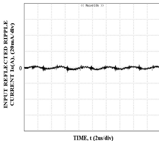
Figure 12: Input reflected ripple current, i_S , through a 12\mu H source inductor at nominal input voltage and rated load current (20 mA/div).
