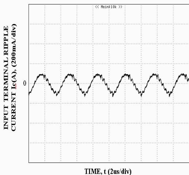
Figure 11: Input Terminal Ripple Current, i_C , at full rated output current and nominal input voltage with 12\mu H source impedance and 33\mu F electrolytic capacitor (200 mA/div).
