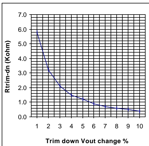
Fig 6 Trim Down Resistance for reference chart
