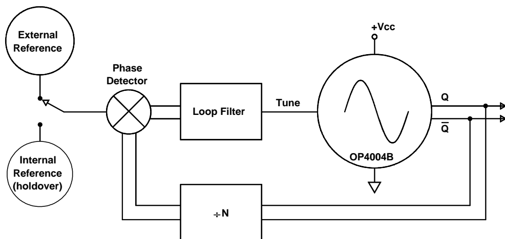
PLL for Generating a High Stability 625 MHz Clock
