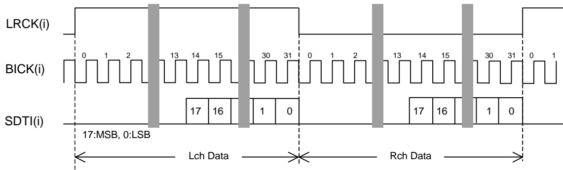
Figure 9. Mode 1 Timing
