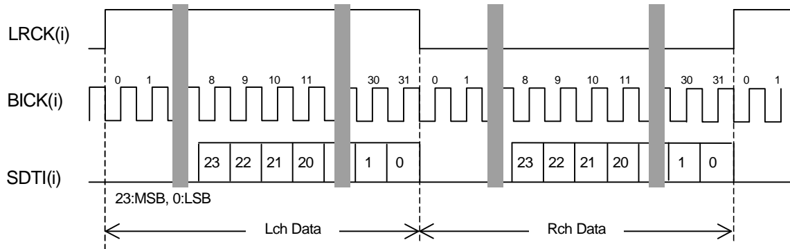
Figure 11. Mode 3 Timing
