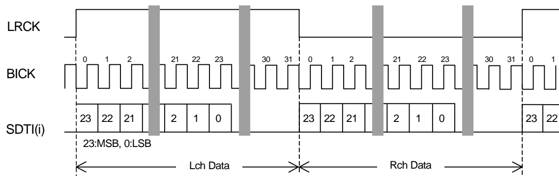
Figure 12. Mode 4, 6 Timing
