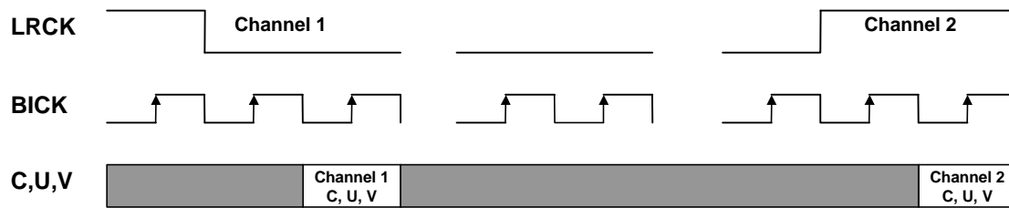
Figure 7. Audio routing, DIF modes 5 and 7 (I 2 S)
