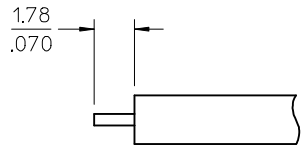
RG405 CABLE PREP
