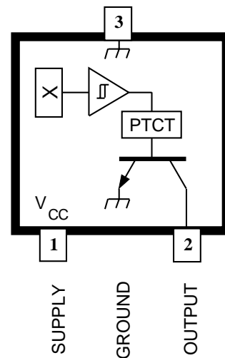
Dwg. PH-003-4
