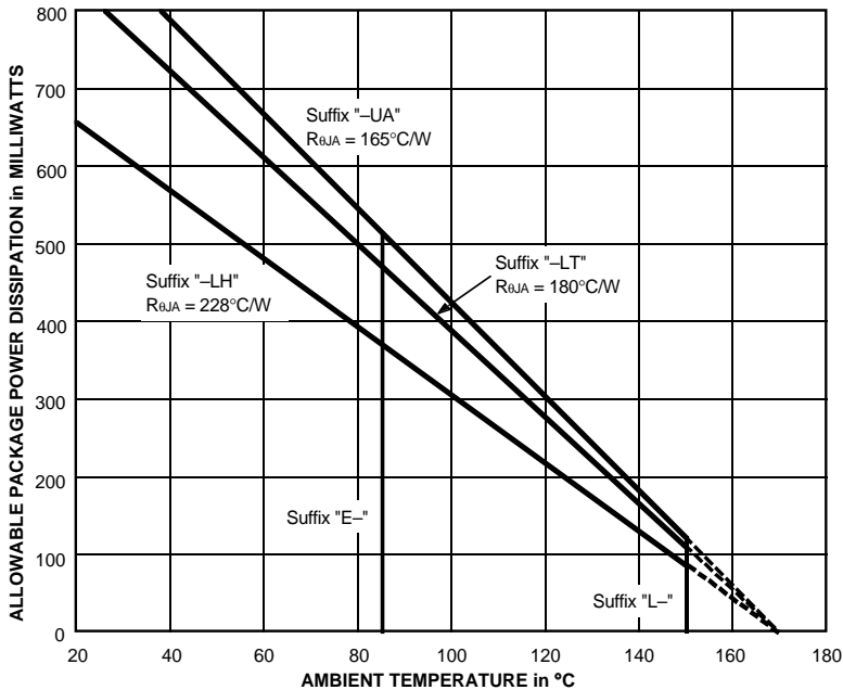
Dwg. GH-046-2D
