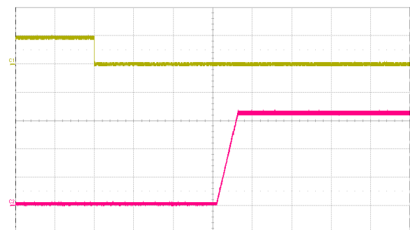
Fig. 10: Turn-on transient at full rated load current (resistive) plus 10,000 \mu\text{F} at V_{in} = 48\text{V} , triggered via ON/OFF pin. Top trace: ON/OFF signal (5 V/div.). Bottom trace: output voltage (1 V/div.). Time scale: 20 ms/div.
