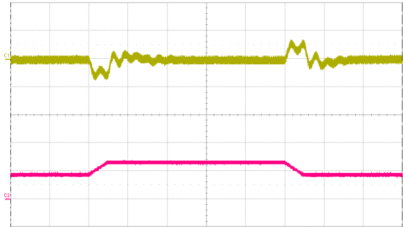
Fig. 11: Output voltage response to load current step change (18A – 27A – 18A) at V_{in} = 48 V. Top trace: output voltage (200 mV/div.). Bottom trace: load current (20 A/div.). Current slew rate: 0.1 A/ \mu s. C_o = 1 \mu F ceramic + 10 \mu F tantalum. Time scale: 200 \mu s/div.
