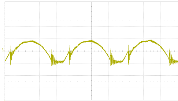
Fig. 13: Output voltage ripple (20 mV/div.) at full rated load current into a resistive load with C_o = 10 \mu F tantalum + 1 \mu F ceramic and V_{in} = 48 V. Time scale: 1 \mu s/div.
