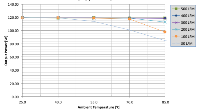
Fig. 6: Power derating vs. ambient air temperature and airflow rates for UIE48T36033 converter with baseplate equipped with .45" finned heatsink mounted vertically with air flowing from pin 3 to pin 1, MOSFET temperature \leq 125^{\circ}\text{C} , V_{in}=48\text{V}
