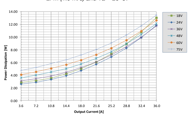
Fig. 8: Power dissipation vs. load current and input voltage for UIE48T36033 converter w/o baseplate mounted vertically with air flowing from pin 3 to pin 1 at a rate of 300 LFM (1.5 m/s) and T_a = 25^{\circ}\text{C} .
