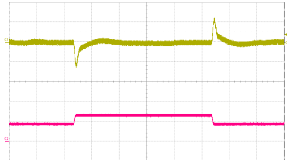
Fig. 12: Output voltage response to load current step change (18A – 27A – 18A) at V_{in} = 48 V. Top trace: output voltage (200 mV/div.). Bottom trace: load current (20 A/div.). Current slew rate: 1 A/ \mu s. C_o = 1 \mu F ceramic + 10,000 \mu F + 10 \mu F tantalum. Time scale: 200 \mu s/div.
