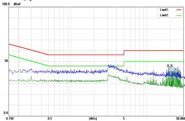
Fig. 20: Vin- Peak Detector EMI waveform
