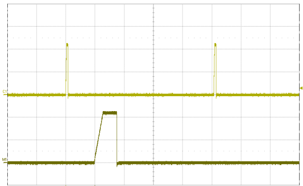
Fig. 17: Load current (top trace, 20 A/div, 100 ms/div.) into a 10 mΩ short circuit during restart, at Vin = 48 V. Bottom trace (20 A/div., 10 ms/div.) is an expansion of the on-time portion of the top trace
