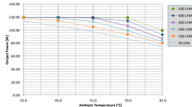
Fig. 4: Power derating vs. ambient air temperature and airflow rates for UIE48T36033 converter w/o baseplate mounted vertically with air flowing from pin 3 to pin 1, MOSFET temperature \leq 125^\circ\text{C} , V_{in}=24\text{V}
