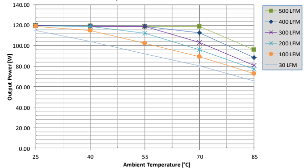
Fig. 2: Power derating vs. ambient air temperature and airflow rates for UIE48T36033 converter w/o baseplate mounted vertically with air flowing from pin 3 to pin 1, MOSFET temperature \leq 125^\circ\text{C} , V_{in}=48\text{V}
