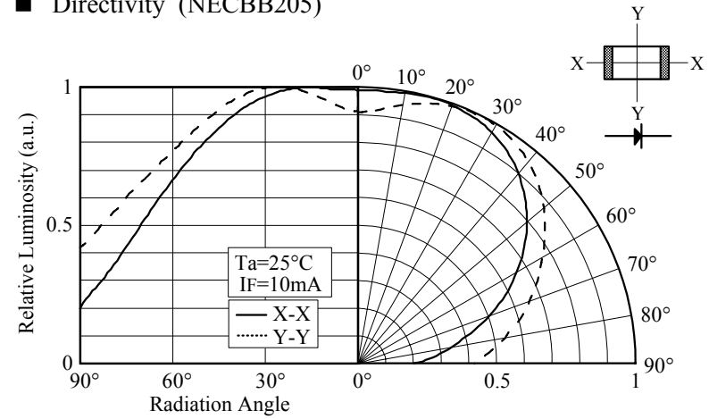
■ Directivity (NECBB205)
