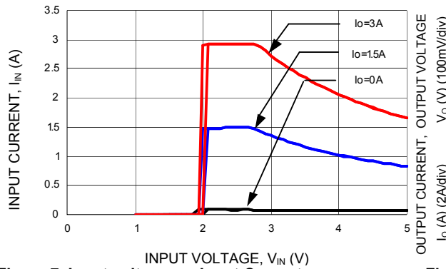
Figure 7. Input voltage vs. Input Current (V out = 2.5Vdc).
