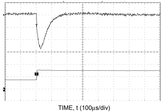
Figure 12. Transient Response to Dynamic Load Change from 50% to 100% of full load (V o = 3.3Vdc, C ext = 2x150 μF Polymer Capacitors).
