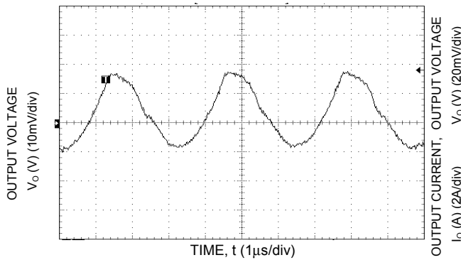
Figure 9. Typical Output Ripple and Noise (V IN = 5.0V dc, V o = 3.3Vdc, I o = 3A).
