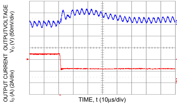
Figure 13. Transient Response to Dynamic Load Change from 100% of 50% full load ( V_o = 3.3\text{ Vdc} , C_{ext} = 2 \times 150\ \mu\text{F} Polymer Capacitors).
