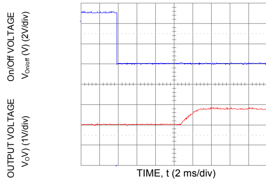
Figure 17 Typical Start-Up using Remote On/off with Prebias ( V_{in} = 3.3\text{Vdc} , V_o = 1.8\text{Vdc} , I_o = 1\text{A} , V_{bias} = 1.0\text{Vdc} ).
