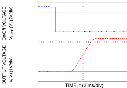
Figure 15. Typical Start-Up Using Remote On/Off with Low-ESR external capacitors ( 7 \times 150\ \mu\text{F} Polymer) ( V_{in} = 5\text{Vdc} , V_o = 3.3\text{Vdc} , I_o = 5.0\text{A} , C_o = 1050\ \mu\text{F} ).
