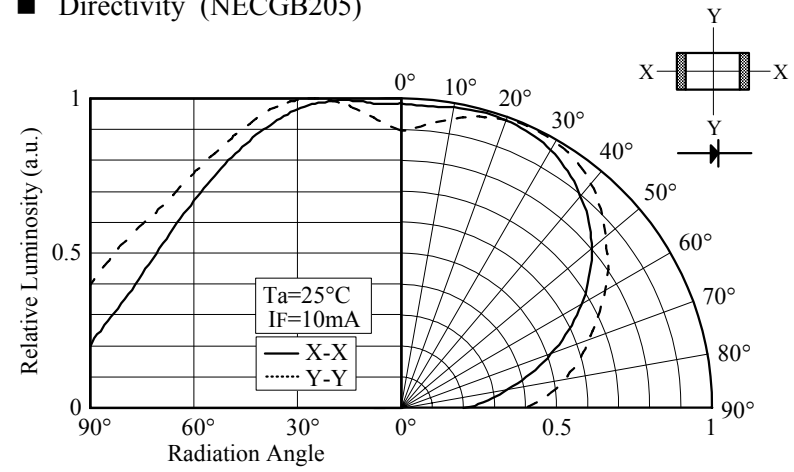
■ Directivity (NECGB205)
