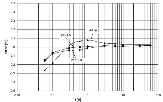
Graph 10: Error as a % of reading for PF=1, PF=-0.8, PF=0.5 at 25°C – Channel I2
