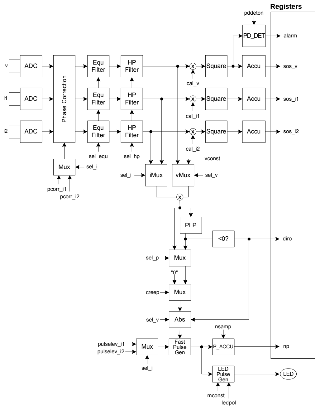
Figure 3: AFE block diagram
