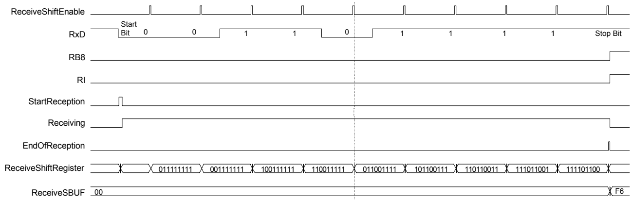
Figure 25: Receiving in mode 1 and mode 2: Here the bit stream '0'+01101111' is received (see signal ReceivedDataBit), that is: start bit + F6h. The start bit is the first 0-pulse of signal RxD, that is when signal ReceivingStartbit is active.
