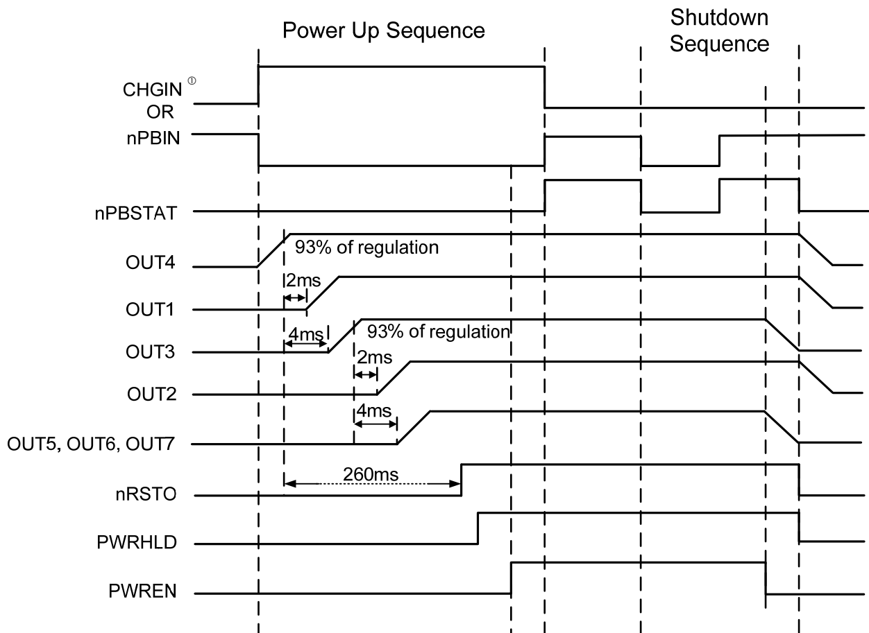
Figure 3: Enable/Disable Sequence
