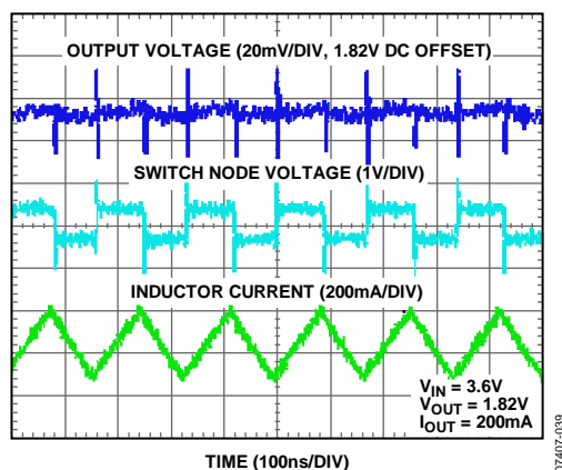
Figure 52. Typical PWM Operation
