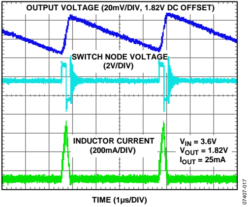
Figure 49. PFM Mode Operation
