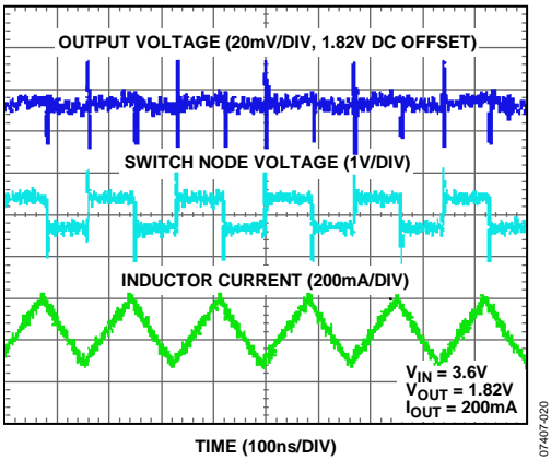
Figure 50. PWM Mode Operation
