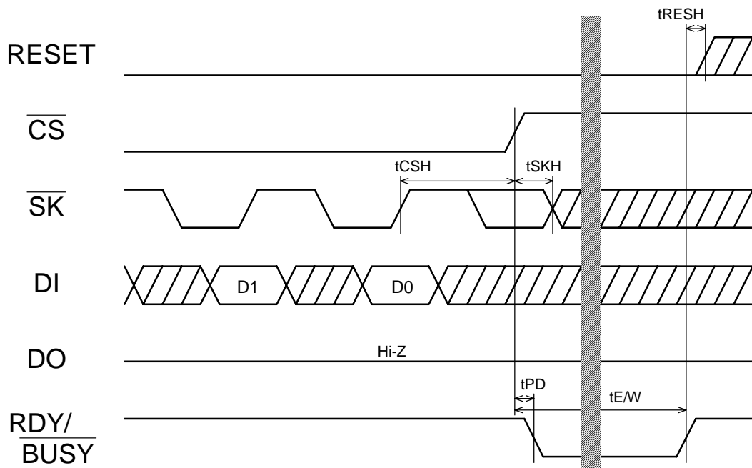
PAGE WRITE Ready / Busy Signal Output (RDY/ BUSY pin)
