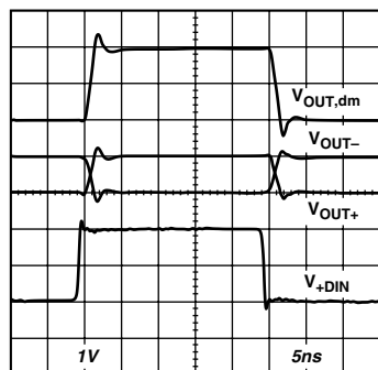
TPC 41. Large Signal Transient Response, G = 1
