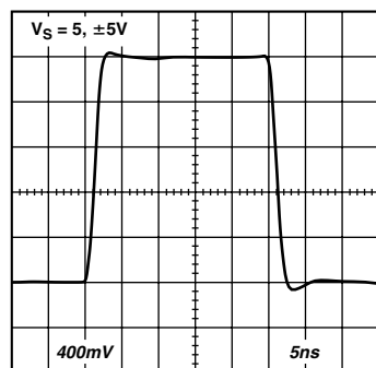
TPC 44. Large Signal Transient Response, G = 2
