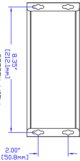
BOTTOM VIEW
