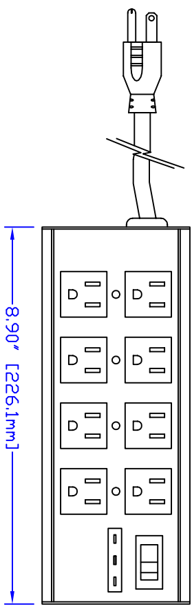
TOP VIEW
