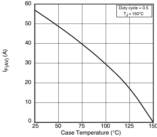
Figure 31. Maximum Average Forward Current vs. Case Temperature
