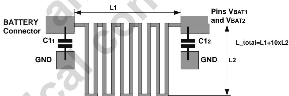
Figure 25. PCB Wire Inductance Example 2
