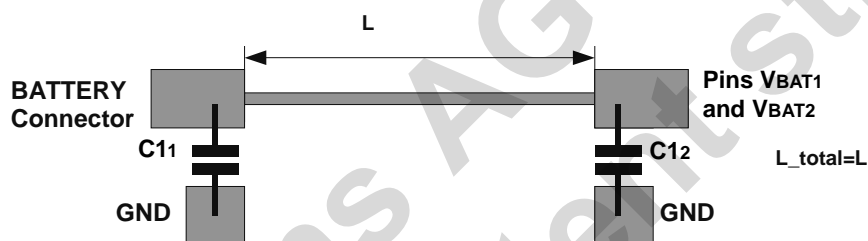
Figure 24. PCB Wire Inductance Example 1
