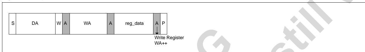
Figure 19. Byte Write
