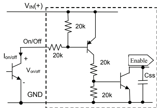
Figure 27. Remote On/Off Implementation.
