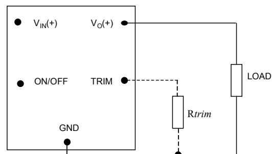
Figure 28. Circuit configuration to program output voltage using an external resistor.
