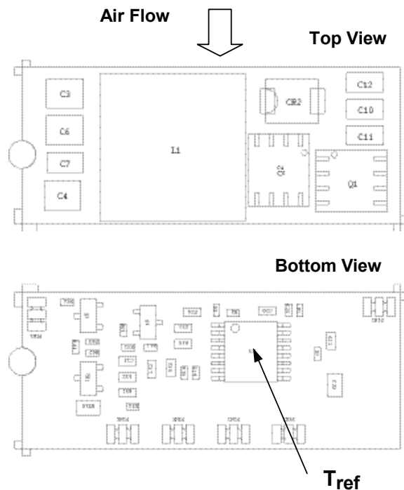
Figure 32. T_{ref} Temperature measurement location.
