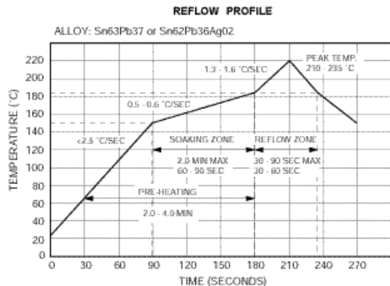
Figure 35. Reflow Profile.
