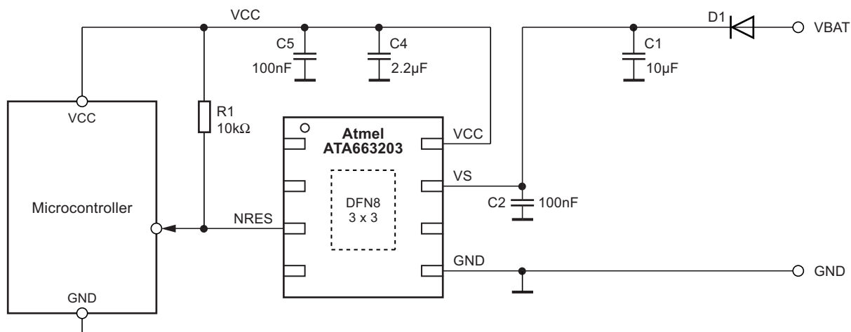
Figure 4-2. Typical Application Circuit Atmel ATA663203
