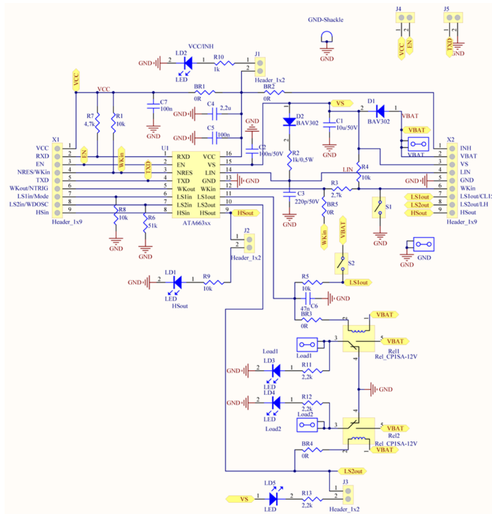
Figure 5-1. Board Schematic
