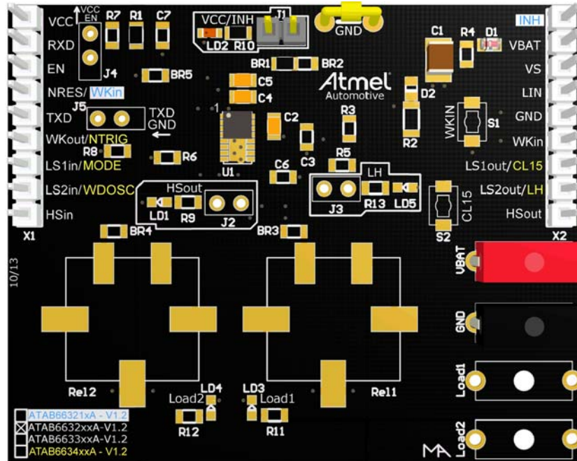
Figure 7-1. Atmel ATA663203 (Voltage Regulator)
