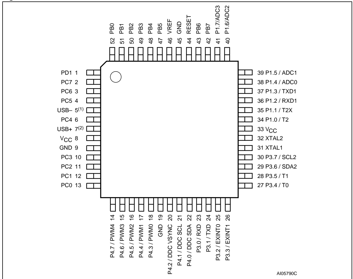
Figure 3. TQFP52 Connections
