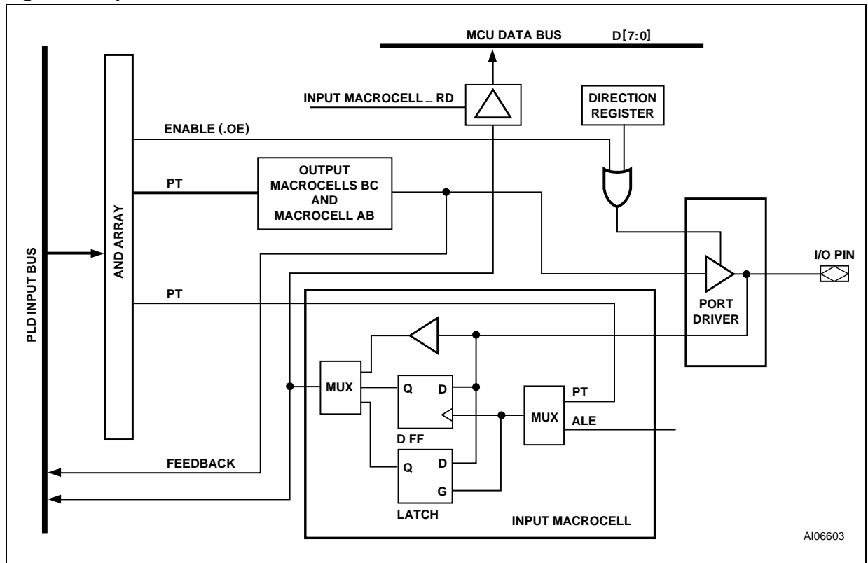
Figure 62. Input Macrocell
