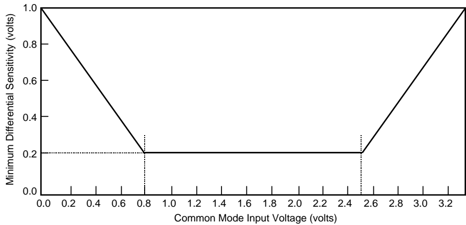
Figure 45. Differential Input Sensitivity Over Entire Common Mode Range
