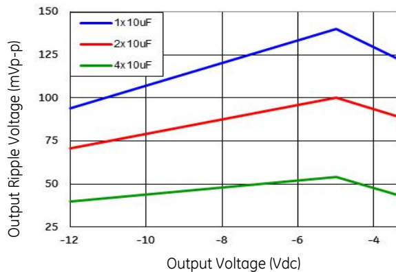
Figure 62. Output ripple with 1x10 \mu F, 2x10 \mu F & 4x10 \mu F output ceramic capacitors (max load).
