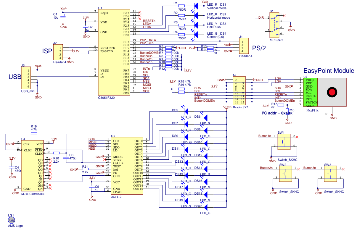
Figure 5: AS5013_DB_2.1 Schematics
