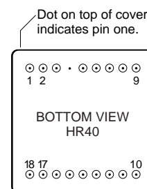
FIGURE 3: PIN OUT
