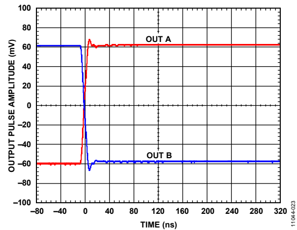
Figure 9. Small Signal Output Transient Response, Normalized to 0 V, 10 ns Rise Time, 10 ns Fall Time, 1 μs Pulse Width, 10% Duty Cycle
