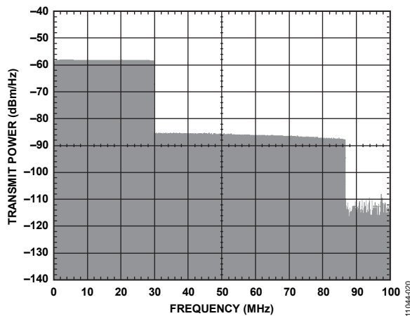
Figure 5. G.hn Transmit Spectrum, 16 dBm into 40 Ω Differential
