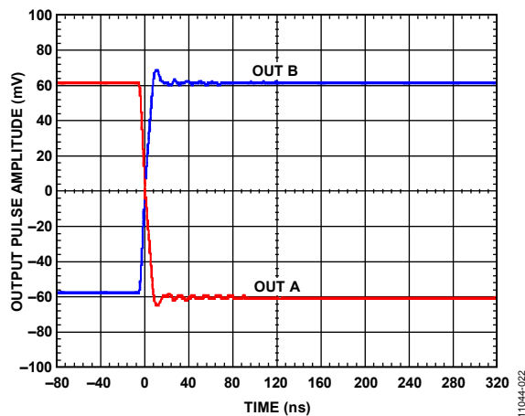
Figure 6. Small Signal Output Transient Response, Normalized to 0 V, 10 ns Rise Time, 10 ns Fall Time, 1 μs Pulse Width, 10% Duty Cycle
