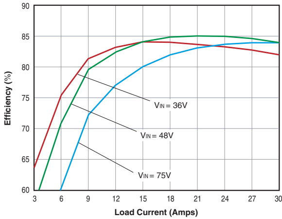
USQ-1.8/30-D48 Efficiency vs. Line Voltage and Load Current
