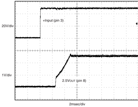
Start-Up from VIN (VIN = 48V, IOUT = 30A, COUT = 10µF tantalum || 1µF ceramic.)
