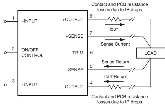
Figure 14. Remote Sense Circuit Configuration
