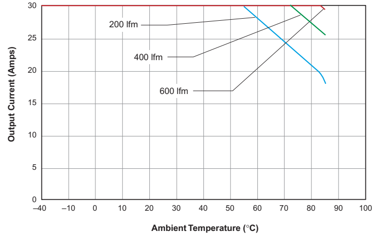
USQ-3.3/30-D48: Output Current vs. Ambient Temperature (Transverse air flow, pin 1 to pin 3; VIN = 48V, 1/4" heat sink.)
