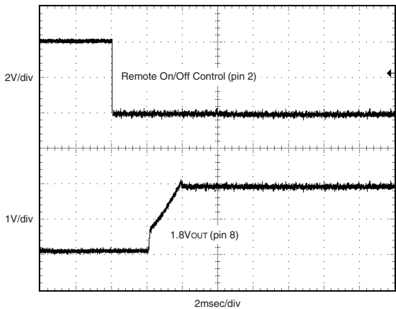
Start-Up from Remote On/Off Control (VIN = 48V, IOUT = 30A, COUT = 10μF tantalum || 1μF ceramic.)
