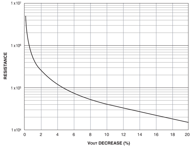
Figure 13. USQ-1.5 to USQ-15 Trim-Down Resistance vs. % Decrease Vout
