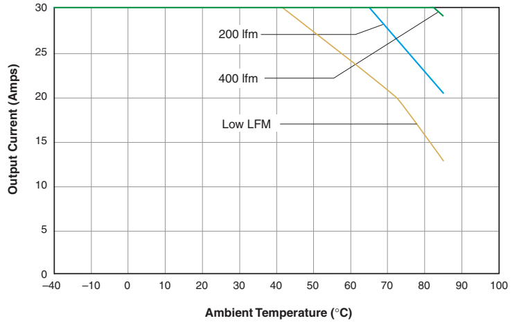
USQ-1.8/30-D48: Output Current vs. Ambient Temperature (Transverse air flow, pin 1 to pin 3; VIN = 48V, no heat sink.)
