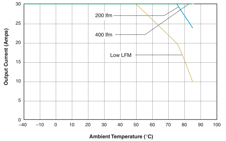
USQ-2.5/30-D48: Output Current vs. Ambient Temperature (Longitudinal air flow, pin 1 to pin 3; VIN = 48V, 1/4" heat sink.)
