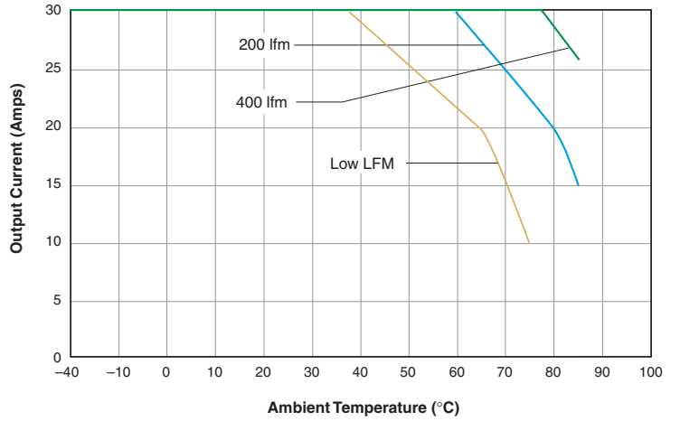
USQ-2.5/30-D48: Output Current vs. Ambient Temperature (Transverse air flow, pin 1 to pin 3; VIN = 48V, no heat sink.)
