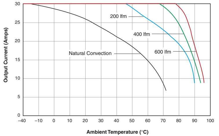
USQ-1.2/30-D48: Output Current vs. Ambient Temperature (Transverse air flow, pin 1 to pin 3; V IN = 48V, no heat sink.)
