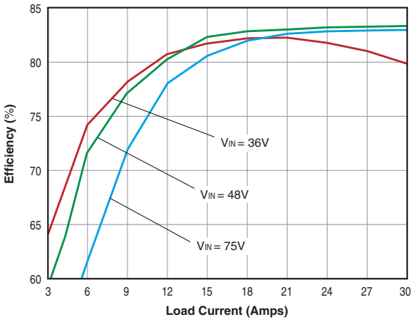
USQ-1.5/30-D48 Efficiency vs. Line Voltage and Load Current
