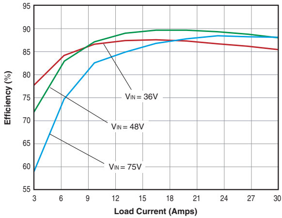
USQ-3.3/30-D48 Efficiency vs. Line Voltage and Load Current
