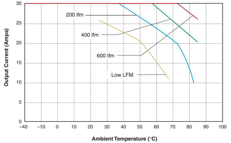
USQ-3.3/30-D48: Output Current vs. Ambient Temperature (Transverse air flow, pin 1 to pin 3; VIN = 48V, no heat sink.)
