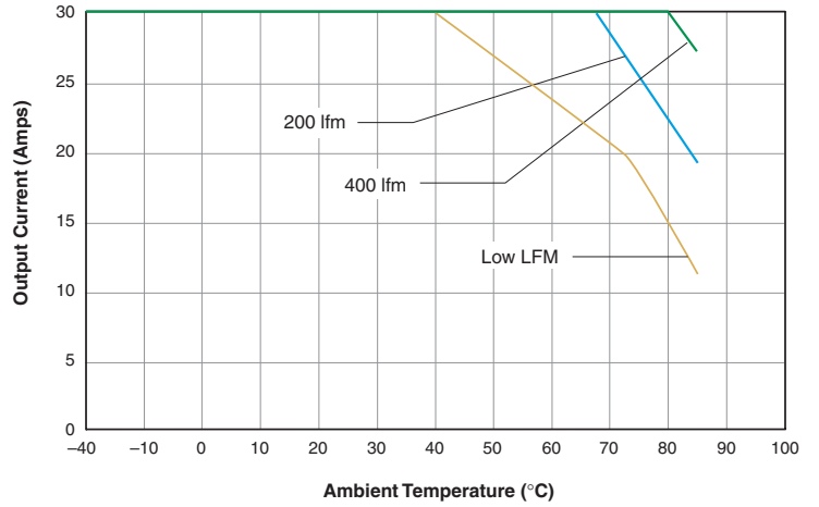
USQ-1.5/30-D48: Output Current vs. Ambient Temperature (Transverse air flow, pin 1 to pin 3; VIN = 48V, no heat sink.)
