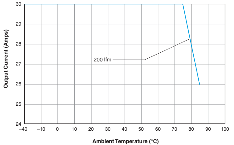
USQ-1.8/30-D48: Output Current vs. Ambient Temperature (Transverse air flow, pin 1 to pin 3; VIN = 48V, 1/4" heat sink.)
