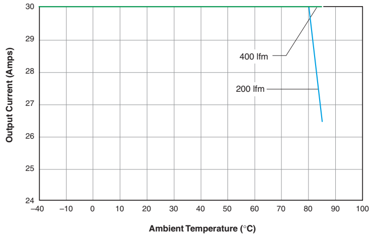
USQ-1.8/30-D48: Output Current vs. Ambient Temperature (Longitudinal air flow, pin 1 to pin 3; VIN = 48V, 1/2" heat sink.)
