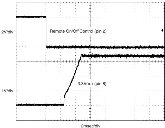
Start-Up from Remote On/Off Control (VIN = 48V, IOUT = 30A, COUT = 10µF tantalum || 1µF ceramic.)
