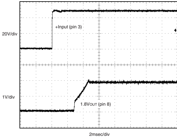
Start-Up from VIN (VIN = 48V, IOUT = 30A, COUT = 10μF tantalum || 1μF ceramic.)
