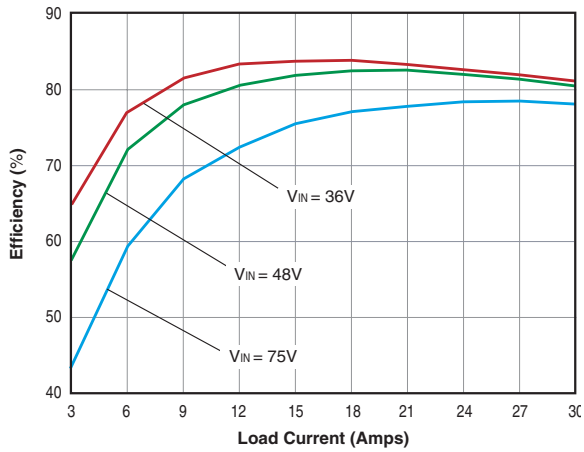
USQ-1.2/30-D48 Efficiency vs. Line Voltage and Load Current
