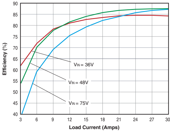
USQ-2.5/30-D48 Efficiency vs. Line Voltage and Load Current
