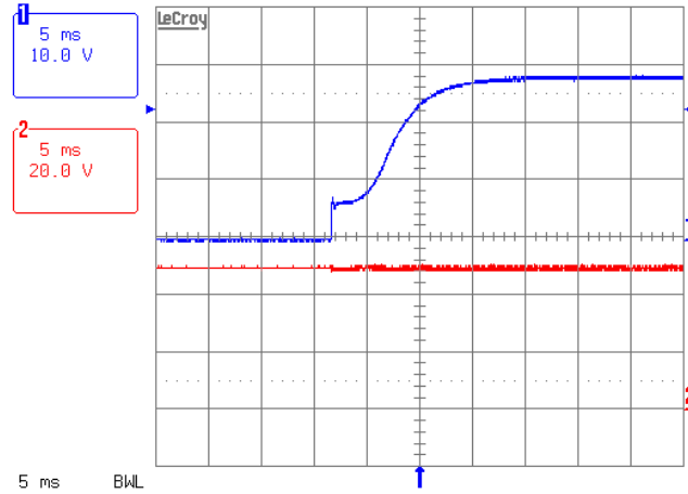
Figure J: Start-up using the on-off enable pin. I_L=12.5\text{Amps} , C_{out}=220\text{ }\mu\text{F} , V_{in}=48\text{ VDC} .
