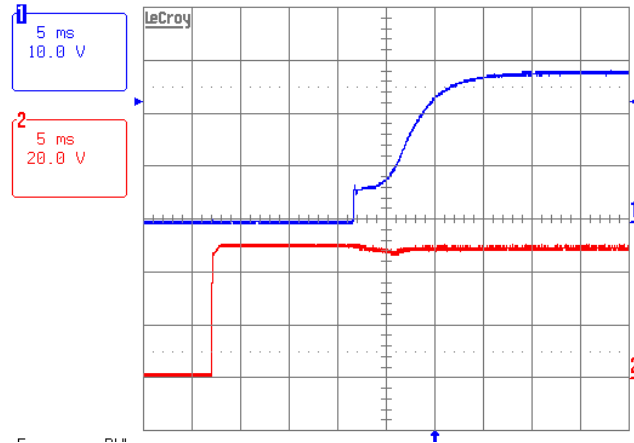
Figure K: Start-up using V_{cc} . I_L=12.5\text{ Amps} , C_{out}=220\text{ }\mu\text{F} , V_{in}=48\text{ VDC} .
