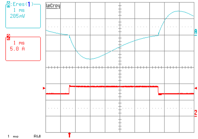
Figure M: Output voltage response to load current step-change (7.5A – 10A – 7.5A) at V_{in} = 48\text{ V} . Current slew rate: 1.0 A/ \mu\text{s} . C_o = 4700\text{ }\mu\text{F} aluminum electrolytic.
