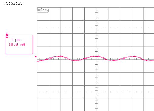
Figure U: Measurement of Ic with Vcc II = 12.5Amps, Cout = 220 μF, Vin = 48 VDC.
