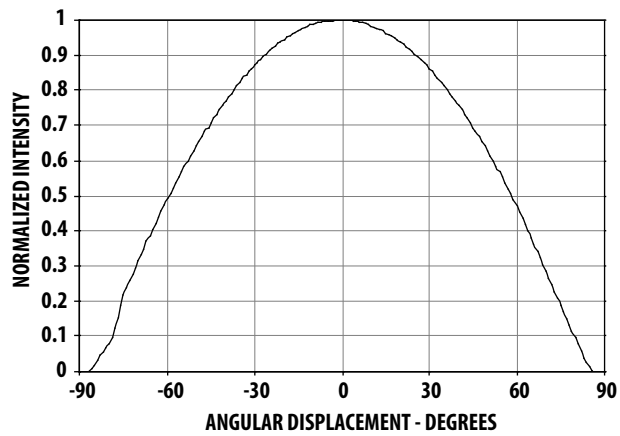
Figure 6. Radiation pattern.
