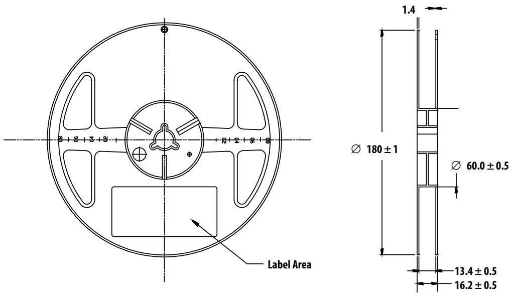
Figure 14. Reel Dimension
