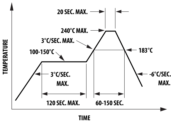
Figure 11. Recommended leaded reflow soldering profile
