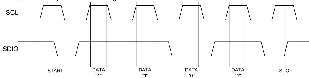
Figure 26 - I 2 C Interface Start/Stop and Data Timing
