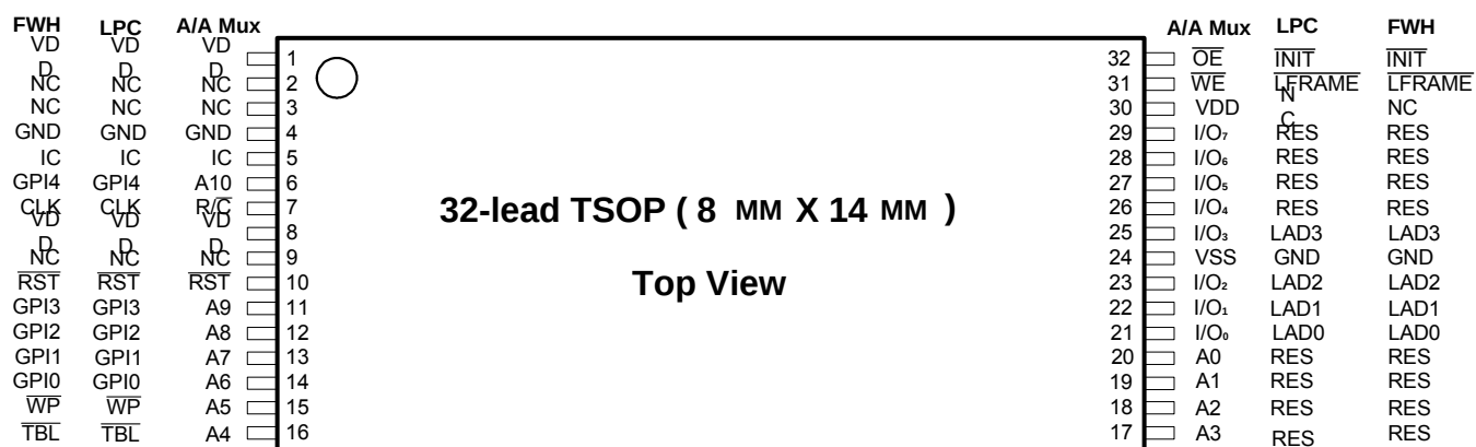
Figure 2: 32-Pin TSOP
