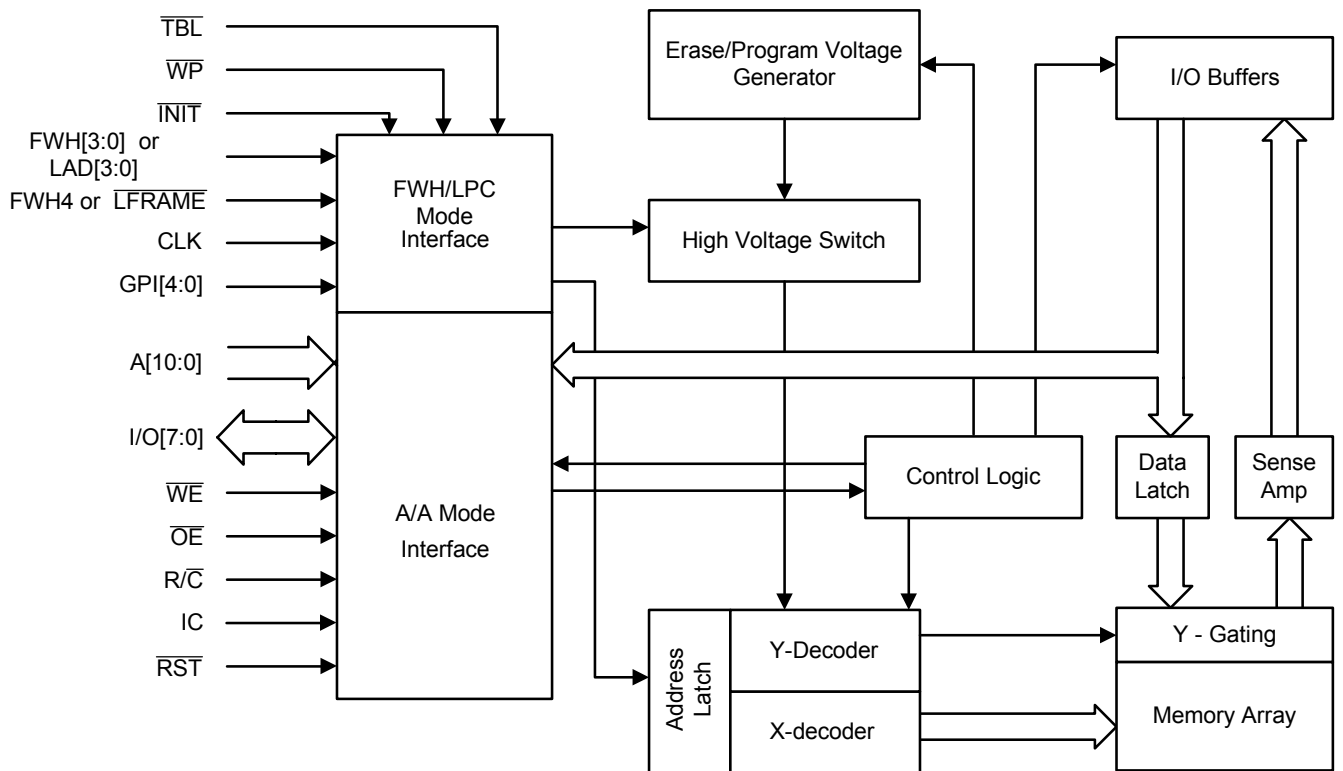
Figure 3: BLOCK DIAGRAM
