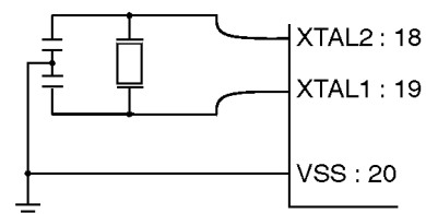
Figure 5. Crystal Oscillator.
