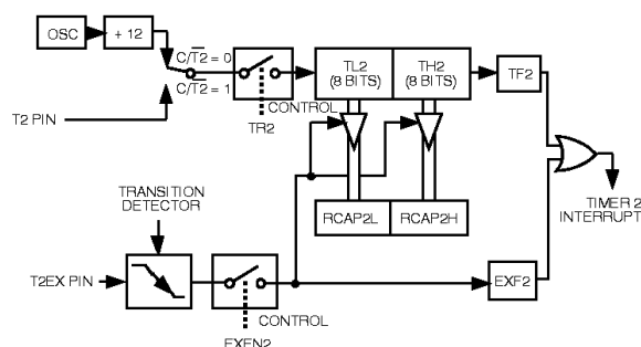
Figure 7. Timer 2 in Capture Mode.
