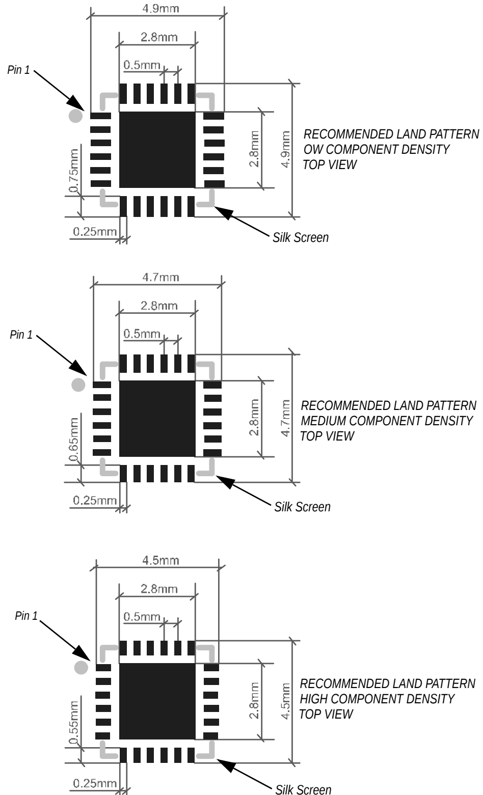
Figure 46. AS3421 PCB Footprint Recommendation
