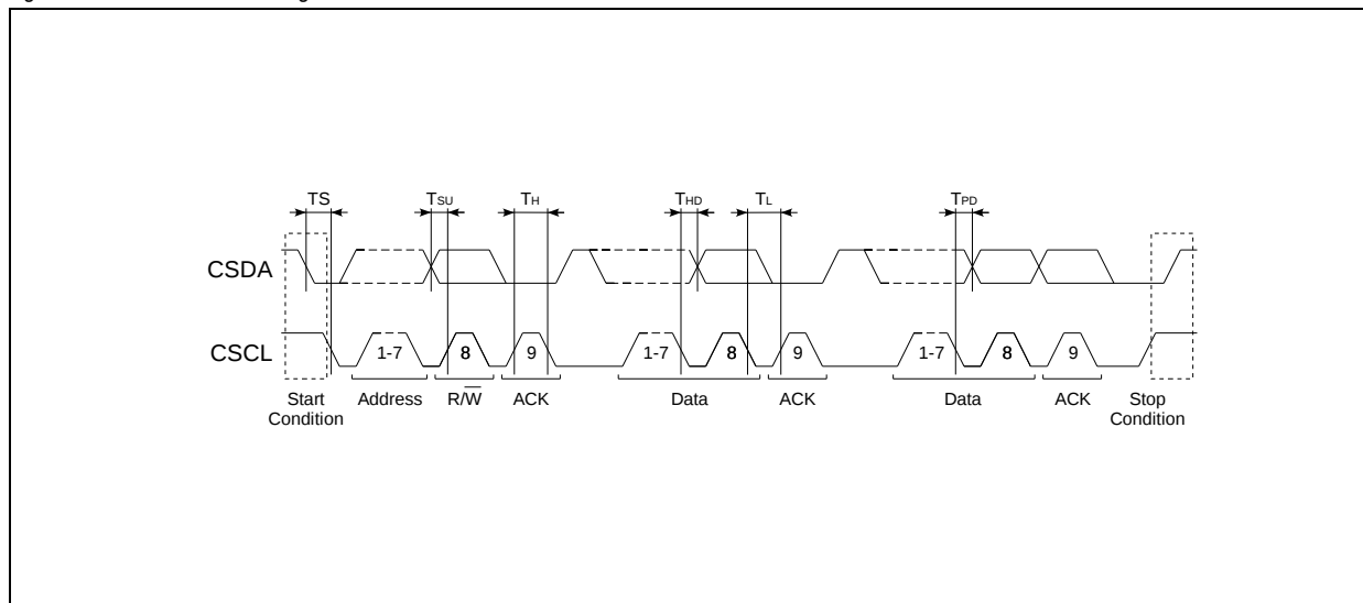
Figure 34. 2-Wire Serial Timing
