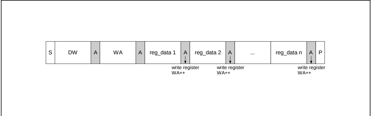
Figure 30. Page Write
