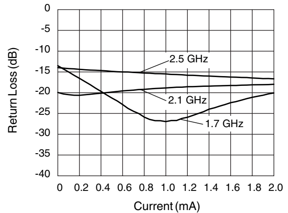
Output Return Loss vs. Current Control
