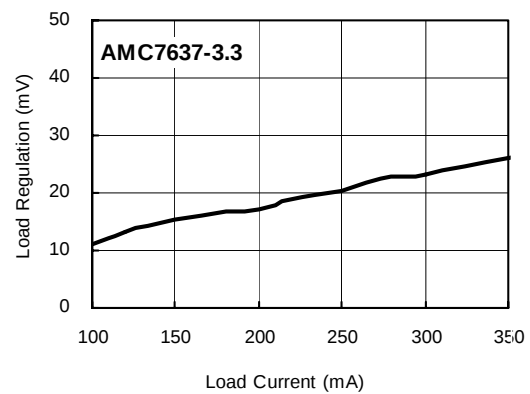
Load Regulation vs. Load Current
